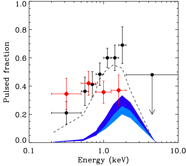
FIG. 3.— Pulsed fraction as a function of energy for the Q-mode (black dots) and B-mode (red diamonds) as derived from the 3D-ML analysis. Errors bars are at 1\sigma , the upper limit at 2\sigma . The blue regions indicate the comparison with model atmosphere predictions for the most likely geometry of PSR B0943+10 (see Sect. 4.3). The dashed line is the pulsed fraction computed by Storch et al. (2014), corrected to account for the unpulsed non-thermal emission.
