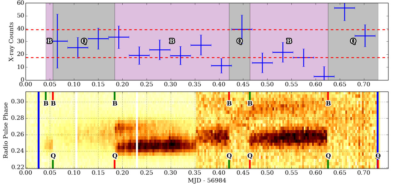
FIG. 1.— Radio and X-ray lightcurves for Session 5. Top panel: XMM-Newton EPIC pn counts from PSR B0943+10 in the 0.2–10 keV band, binned in 3670-s intervals and corrected for the exposure reduction due to the exclusion of high-background periods. The radio-identified B/Q-modes are shown by the shaded regions. The dashed lines show the average B/Q-mode count levels determined from the entire 2014 data set. Bottom panel: Radio pulse profiles, each 300 s, zoomed-in on a narrow range around the main pulse peak. The sudden transition in profile shape and noise properties at MJD = 56984.35 is when observing coverage shifted from LOFAR (observing at \sim 150 MHz) to LWA (observing at \sim 60 MHz). Note that the observed brightness of PSR B0943+10 is modulated by both intrinsic effects (the mode switching) as well as the effective sensitivity of the telescope due to the changing source elevation. The start/stop times of B/Q-modes are indicated by the green/red ticks at the top/bottom of the panel. The vertical blue bars indicate XMM-Newton observation start/stop times.
