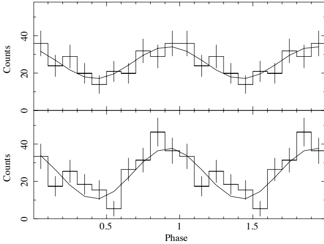
FIG. 5.— Folded pulse profiles in the 0.5-2 keV range for the early-B (top) and late-B (bottom) time intervals (see text). The background has been subtracted. The curves show fits with a constant plus a sinusoid with phase fixed to that of the whole B-mode. The amplitudes of the sinusoids are 8.6 \pm 1.8 and 13.7 \pm 1.9 for the early-B and late-B, respectively, and the constants are 25.6 \pm 1.3 and 24.2 \pm 1.4 .
