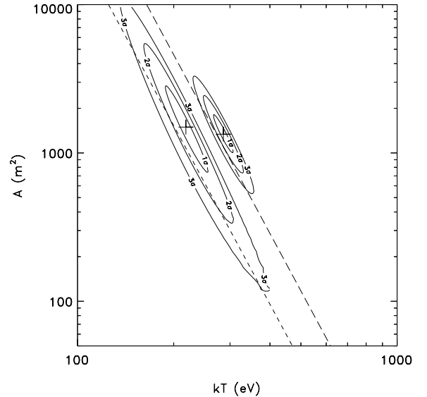
FIG. 7.— Confidence regions ( 1\sigma , 2\sigma , and 3\sigma c.l.) of blackbody temperature and emitting area for the pulsed thermal component of the B-mode (bottom-left contours) and Q-mode (top-right contours). The dashed lines correspond to bolometric luminosities of 10^{29} and 3 \times 10^{29} erg s^{-1} , for a distance of 630 pc.
