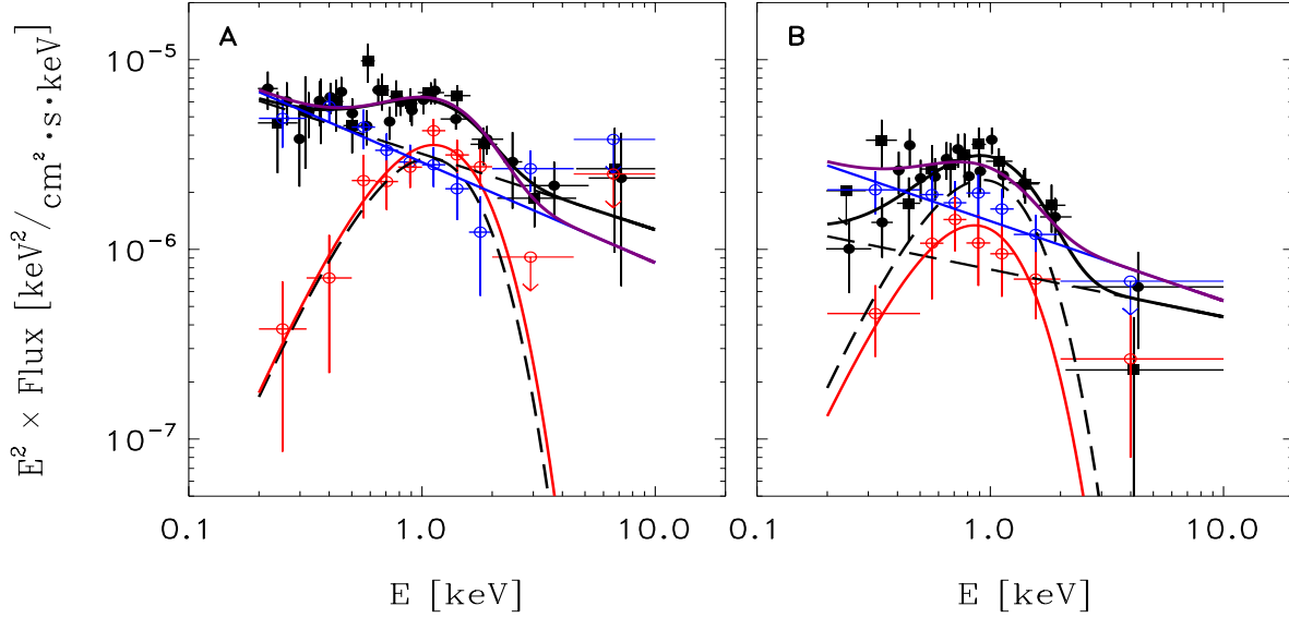
FIG. 4.— Results of the ML spectroscopy for the Q-mode (left panel) and B-mode (right panel). Black lines and points refer to the 2D-ML (circles pn, squares sum of the two MOS, solid lines are the best-fit blackbody plus power law models, dashed lines the individual components). The results of the 3D-ML analysis are in blue for the unpulsed component (data points and best-fit with a single power-law) and in red for the pulsed component (data points and best-fit with a single blackbody). The purple line is the sum of the blue and red lines.
