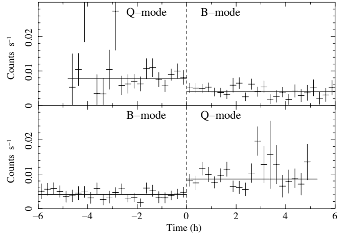
FIG. 6.— Light curves (pn+MOS, background subtracted, 0.2-2.5 keV, time bins of 900 s) obtained by stacking all the Q to B (top panel) and B to Q (bottom panel) mode transitions observed in 2014. The light curves are corrected to take properly into account the exposure time resulting from the different lengths of the time intervals and from the gaps due to the data cleaning. The horizontal lines indicate fits with constant count rates to 6 hr long intervals and have the following values. Q-mode before transition: 0.0078 \pm 0.0006 ( \chi^2_\nu = 0.90 ); B-mode after transition: 0.0040 \pm 0.0003 ( \chi^2_\nu = 0.80 ); B-mode before transition: 0.0041 \pm 0.0003 ( \chi^2_\nu = 0.66 ); Q-mode after transition: 0.0086 \pm 0.0005 ( \chi^2_\nu = 1.17 ).
