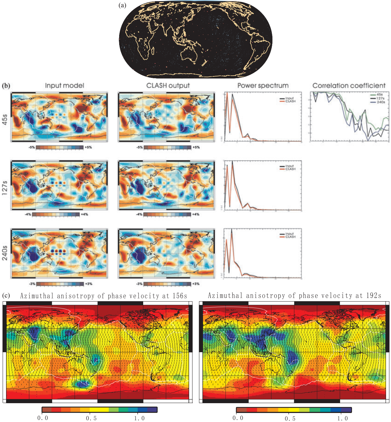
Figure 11. (a) Path coverage used for regionalization of fundamental Rayleigh mode phase velocity. There are about 4318 paths totally. The sources are indicated by red dot. (b) comparison of phase velocity between input model and CLASH results for three different periods 45, 127 and 240 s. Right-hand column: the correlation coefficients of spherical harmonics coefficients. Second column from right-hand side: the comparison of power spectrum. (c) Azimuthal anisotropy of fundamental Rayleigh phase velocity at different periods 156 and 192 s. The bar length corresponds the magnitude of azimuthal anisotropy. The colour scale in the background corresponds to the peak-to-peak amplitude of anisotropy, expressed with respect to the mean phase velocity.
