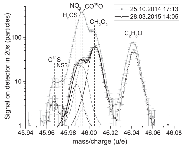
Figure 8. Mass spectra of m/z 46 u/e (row A). Identified species are indicated by dashed lines. In black is shown the signal during the flyby on 2015 March 28 when the signal of CO 2 was comparably low while in grey the typical signal on m/z 46 u/e is shown. For the measurement of March 28, the fit is shown with dash-dotted lines while the cumulative fit is drawn in black.
