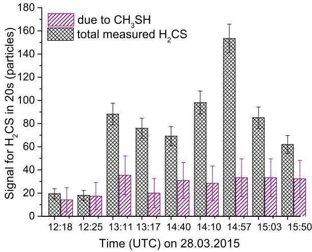
Figure 9. \text{H}_2\text{CS} budget during flyby in 2015 March ( 1\sigma ). For each contribution, 1\sigma error bars are given.
