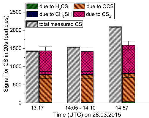
Figure 10. CS budget around the closest approach of the flyby in 2015 March. For each contribution, 1\sigma error bars are given.
