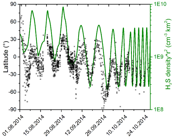
Figure 12. \text{H}_2\text{S} density multiplied by distance to comet squared for the period August 1 to the end of 2014 October together with the sub-spacecraft latitude. Statistical errors are smaller than symbol size.
