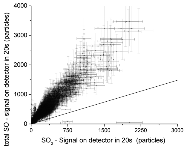
Figure 7. Total measured SO abundance including contribution from fragmentation of SO 2 (black squares). The black line shows the contribution to SO by fragmentation of SO 2 inside DFMS's ion source.
