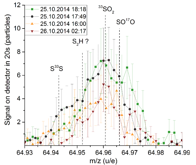
Figure 5. Representative spectra of m/z 65 u/e during 10 km orbits in 2014 October.
