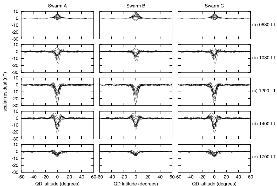
Figure 1. Scalar residual after subtracting main, crustal, magnetospheric and Sq fields for five different days in 2014: (a) 6 July, (b) 25 May, (c) 6 May, (d) 16 April, and (e) 15 March. Indicated local times are approximate and correspond to equator crossings on the dayside of the Earth. They may slightly differ from one satellite to the next (for instance, local time for Swarm B on 6 July was closer to 0700 than to 0630, which could explain why the signal seen by Swarm B is somewhat stronger than that seen by Swarm A and Swarm C).
