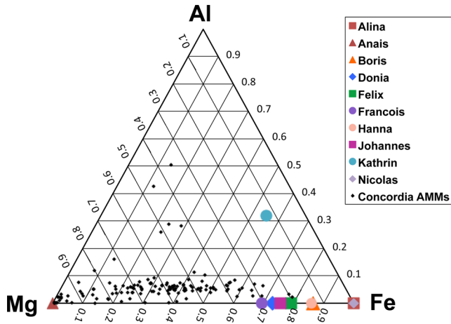
Figure 4. Mg-Al-Fe ternary diagram of the composition of 10 cometary dust particles from comet 67P/Churyumov-Gerasimenko analysed by COSIMA compared to that of 130 micrometeorites from the Concordia micrometeorite collection (data from Hilchenbach et al. 2016, Duprat et al. 2007 and unpublished data).
