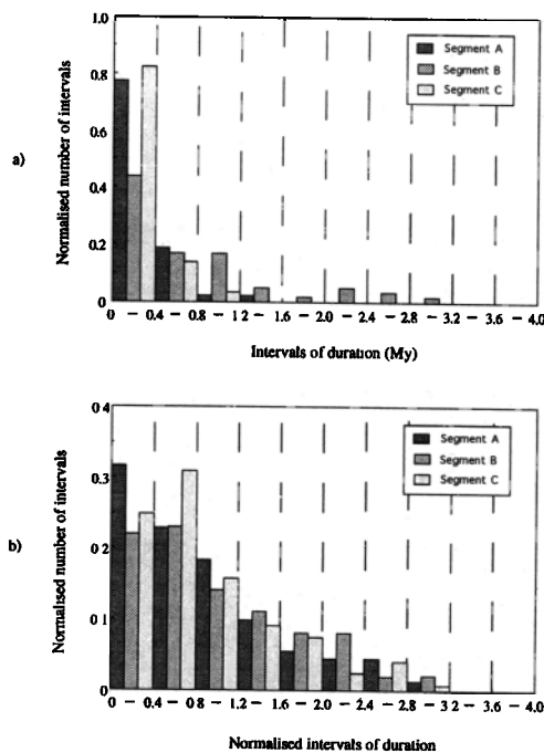
Figure 2. Histograms of duration of the intervals defining the three segments A,B,C. Only the intervals following the Cretaceous superchron have been considered for the segment B. The histograms have been normalized to the total number of intervals within each segment (Fig. 2a). Fig. 2b: same except that the duration of the magnetic intervals has been divided by the time varying estimates of \mu displayed on Fig. 1b.
