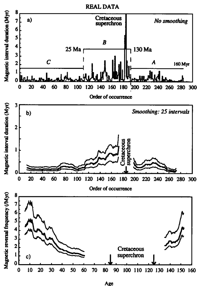
Figure 1. Polarity interval durations as a function of order of occurrence (Fig. 1a,b). The first interval is Brunhes. The raw data is shown on Fig. 1a, and \mu_N(i) for N=25 and k=1 is plotted with its 2\sigma_N=25 errors ( \sigma_N(i)=\mu_N(i)/\sqrt{N} ) on Fig. 1b (except those involving the Cretaceous superchron). Fig. 1c shows \lambda^*_{50} since approximately 160 Myr. We also plotted the curves \lambda_+(i)=1/(\mu_{50}(i)+2\sigma_{50}(i)) and \lambda_-(i)=1/(\mu_{50}(i)-2\sigma_{50}(i)) within which \lambda^*_{50} is expected to fluctuate.
