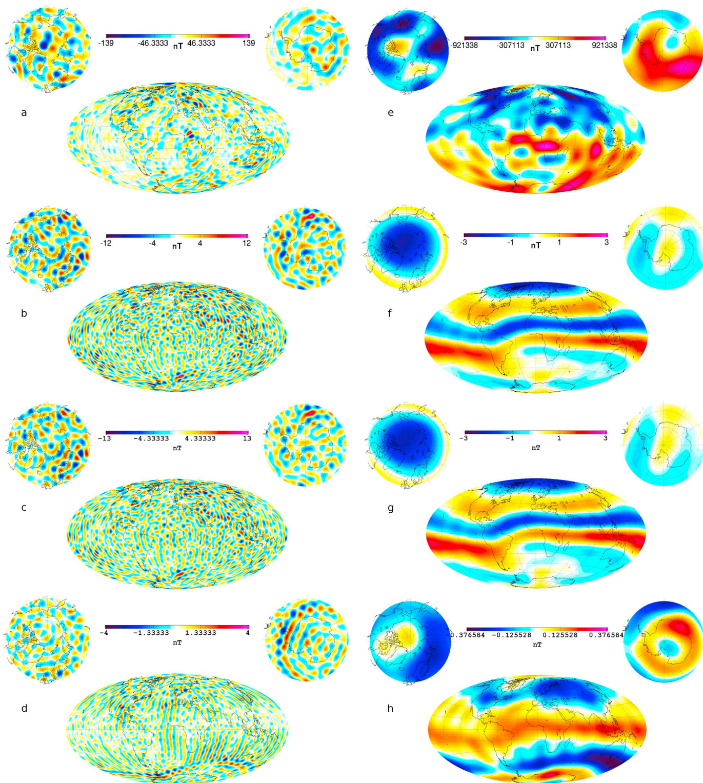
Figure 2. (left) Lithospheric and (right) core field model comparisons: B_r for n = 15\text{--}45 at ground surface from (a) model ASM_V and from (b) ASM_V minus VFM, (c) ASM_V minus VFM_N, and (d) VFM minus VFM_N model differences; B_r for n = 1\text{--}13 , central epoch 22/4/2014 from (e) model ASM_V at the core surface and from (f) ASM_V minus VFM, (g) ASM_V minus VFM_N, and (h) VFM minus VFM_N model differences at satellite altitude.
