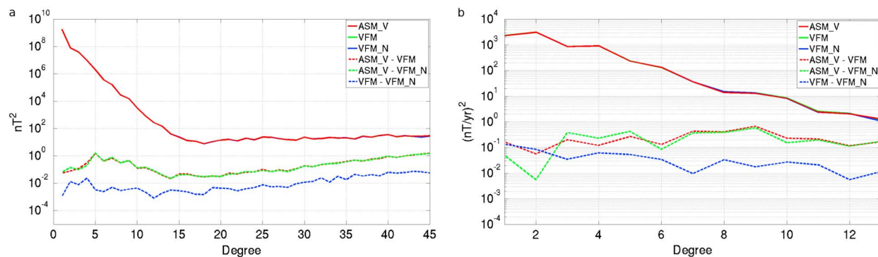
Figure 1. (a) Lowes-Mauersberger spectra of the ASM_V (solid red), VFM (solid green), and VFM_N (solid blue) models for the field of internal origin at the central epoch (22/4/2014), together with the spectra of differences among these models (ASM_V - VFM, dashed red; ASM_V - VFM_N, dashed green; VFM - VFM_N, dashed blue), all at ground surface; (b) Same but for the secular variation spectra.
