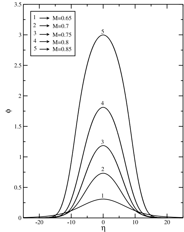
Figure 2. Potential profiles for positive amplitude electron acoustic solitary waves for different Mach numbers. The parameter domain is the same as Figure 1.
