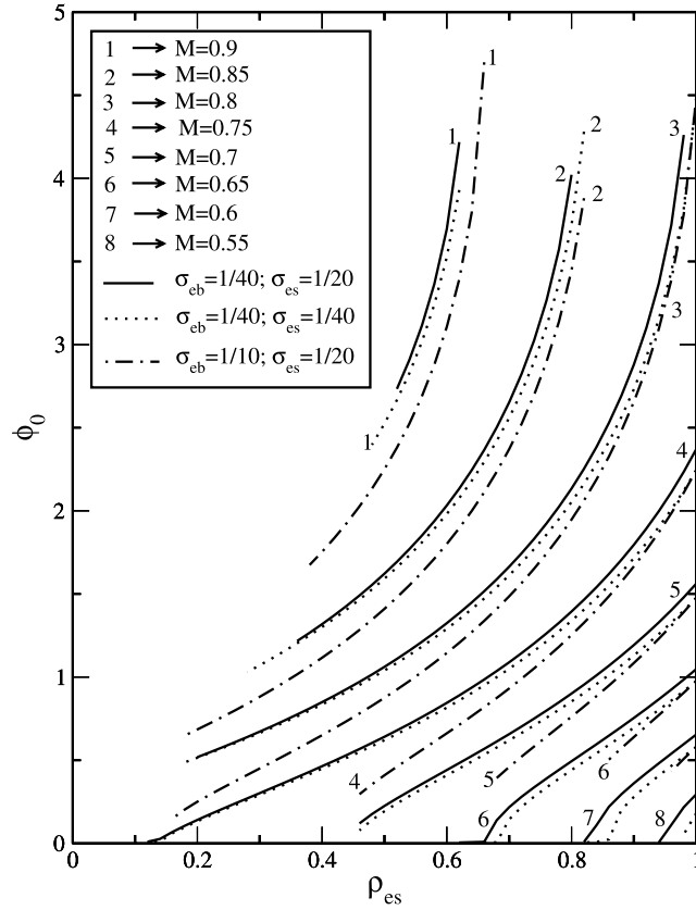
Figure 3. Variation of the amplitude ( \phi_0 ) with bulk electron concentration ( \rho_{es} ) for different M . The solid ( \sigma_{eb} = 1/40 , \sigma_{es} = 1/20 ), dot-dashed ( \sigma_{eb} = 1/10 , \sigma_{es} = 1/20 ), and dotted ( \sigma_{eb} = 1/40 , \sigma_{es} = 1/40 ) curves represent different combinations of beam and bulk electron temperatures. Other parameters are the same as Figure 1.
