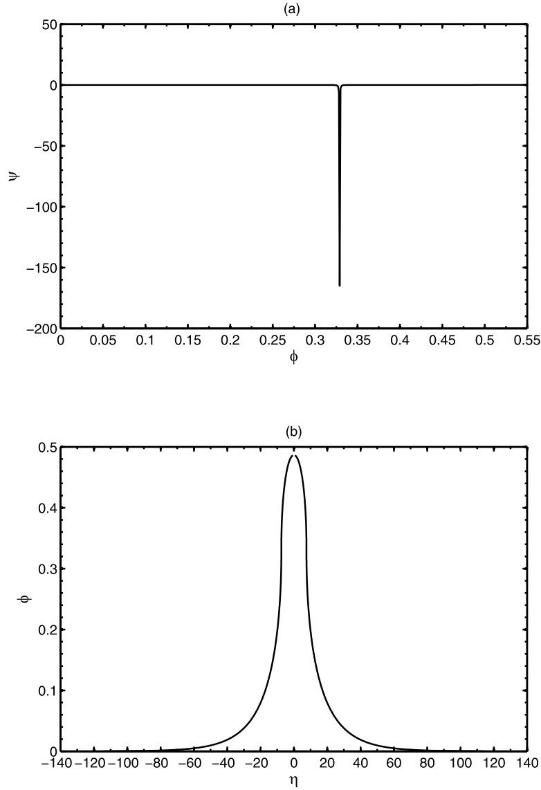
Figure 12. (a) The Sagdeev pseudopotential and (b) the potential profile of the electron acoustic solitary wave in the bow shock transition region. The plasma parameters are \alpha_e = 0.05 , \beta_i = 1/4 , \rho_{es} = 0.98 , \mu_i = 0.85 , \sigma_{es} = 0.1079 , \sigma_{eb} = 0.0863 , M = 0.77 , \theta = 75^\circ , and u_{eb} = 0.0861 .
