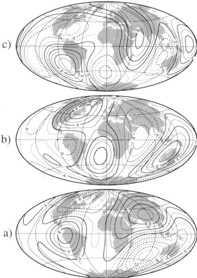
Fig. 6. Vertical component ( \delta \ddot{Z} ) of the 1969 (bottom), 1979 (middle) and 1992 (top) jerks. Contour interval: 2 nT/yr 2 .
