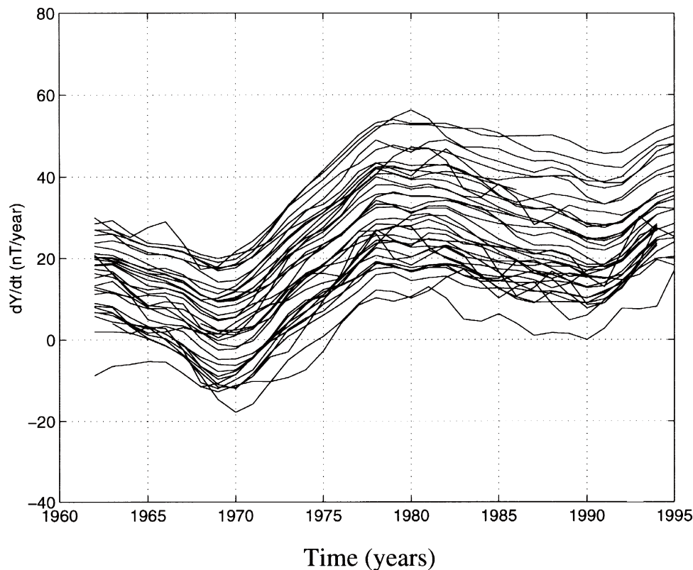
Fig. 2. The secular variation of the Y component observed in the 37 observatories located in Europe.
