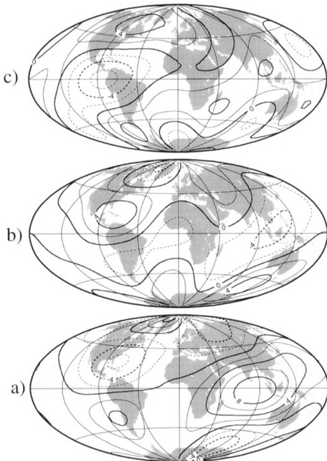
Fig. 4. North component ( \delta \ddot{X} ) of the 1969 (bottom), 1979 (middle) and 1992 (top) jerks. Contour interval: 2 nT/yr 2 .
