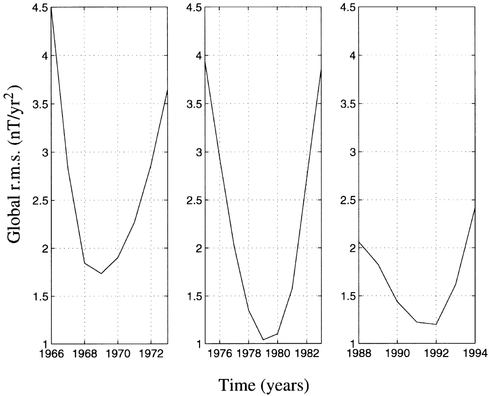
Fig. 3. Variation of the global r.m.s. residual of the secular variation of the Y component around the jerk times. The time for which the global r.m.s. residual is minimum is retained as the date t_0 of the jerk: t_{01} = 1969 , t_{02} = 1979 and t_{03} = 1992 .
