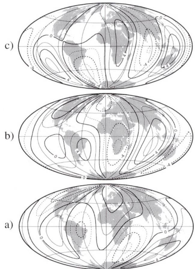
Fig. 5. East component ( \delta \ddot{Y} ) of the 1969 (bottom), 1979 (middle) and 1992 (top) jerks. Contour interval: 2 nT/yr 2 .
