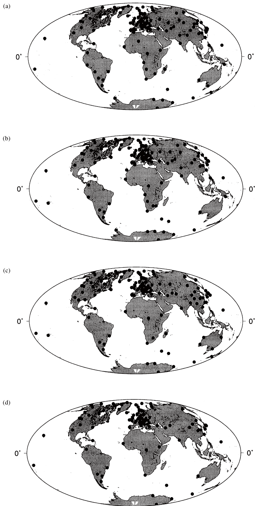
Fig. 1. Distribution of the observatories (a) “dataset 1” used to study the 1969 event; (b) “dataset 2” used to study the 1979 event; (c) “dataset 3” used to study the 1992 event; (d) “dataset 4” with continuous annual mean series from 1960.5 to 1995.5 or 1996.5.
