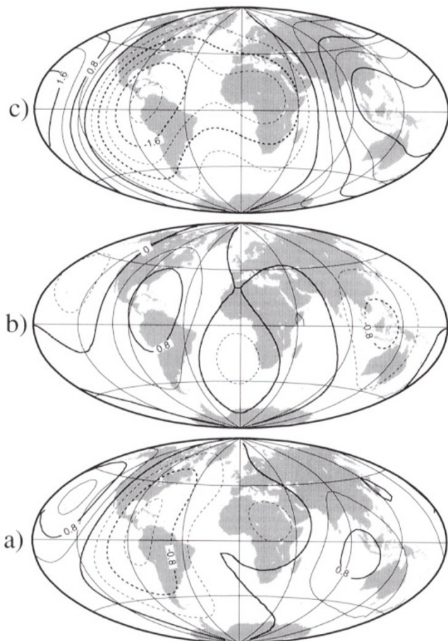
Fig. 7. Poloidal scalar \delta S of the 1969 (bottom), 1979 (middle) and 1992 (top) acceleration jumps. Contour interval: 10^{-4} rad/yr 2 .
