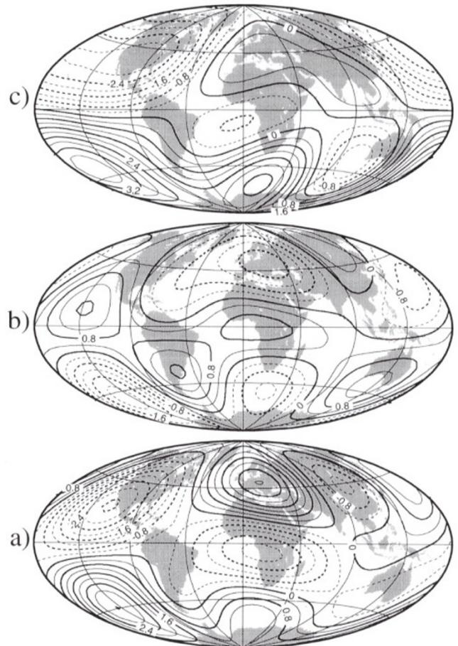
Fig. 8. Toroidal scalar \delta T of the 1969 (bottom), 1979 (middle) and 1992 (top) acceleration jumps. Contour interval: 10^{-4} rad/yr 2 .
