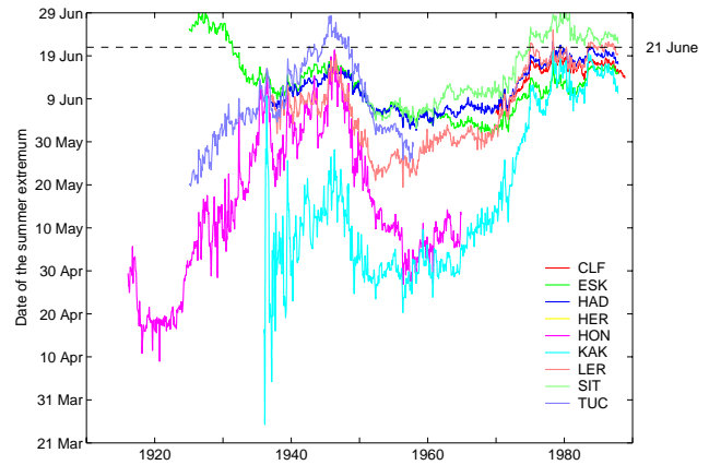
Fig. 9. Time variation of the phase of the annual variation of the X component in nine observatories, computed using a 22-year sliding window, centered. Phases are reckoned as the dates of the summer extrema.
