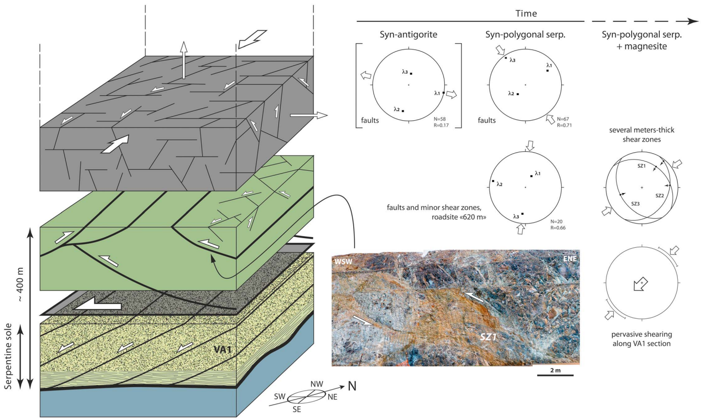
Figure 3. Summary of the results of structural analysis in the Koniambo Massif, adapted from Quesnel et al. [2016a] . (left) Block diagram depicting the style of deformation in the three structural levels identified in the massif. For the upper structural level, the drawing shows the deformation associated with polygonal serpentine. (right) Synthesis of the results of strain inversion as a function of the structural level (vertically) and as a function of the main minerals associated with deformation, which enable a sequence of events to be identified (horizontally). Strain inversion of fault slip data has been carried out with the FaultKin software of Allmendinger et al. [2012] . The parameter R relates to the shape of the strain ellipsoid ( R = (\epsilon_2 - \epsilon_3)/(\epsilon_1 - \epsilon_3) ) hence R equates 0 for pure constriction, 0.5 for plane strain, and 1.0 for pure flattening).
