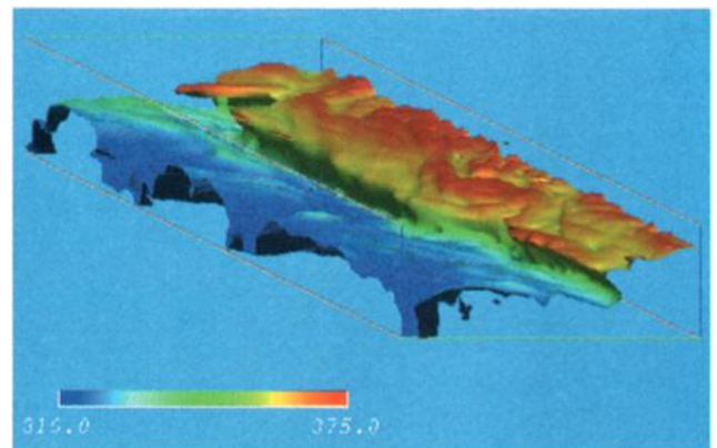
Figure 3. Three-dimensional map of the tropopause defined as the surface PV = -1.2 PVU on July 25, 1998 at 00h UT. The surface is shown within a box extending from 0 to 200 E in longitude, from 5 S to 45 S in latitude and from 600 to 30 hPa in the vertical. Color indicates the potential temperature according to the scale in the lower left corner.
