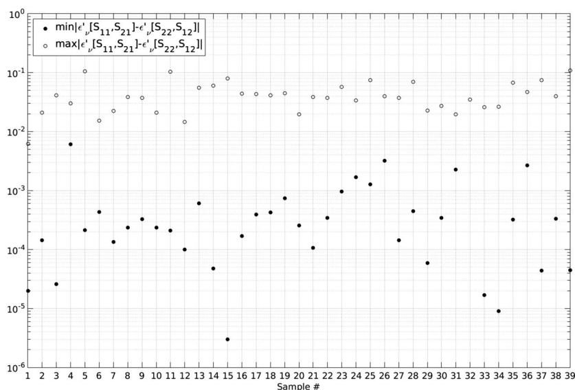
Figure 8. Maximum and minimum differences between \epsilon'_v obtained from S_{11} and S_{21} ( \epsilon'_v [S_{11}, S_{21}] ) and \epsilon'_v obtained from S_{22} and S_{12} ( \epsilon'_v [S_{22}, S_{12}] ) for each sample, taking into account the whole range of frequency. The homogeneity of the samples during the measurements is maintained, as showed by the low values of the differences.
