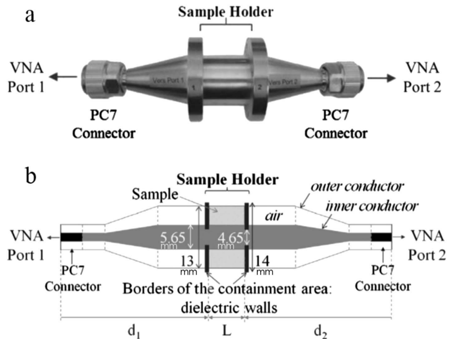
Figure 3. (a) Image and (b) schematic of the conical coaxial cell used to perform the permittivity measurements between 50 MHz and 2 GHz [from Brouet et al. , 2015].
