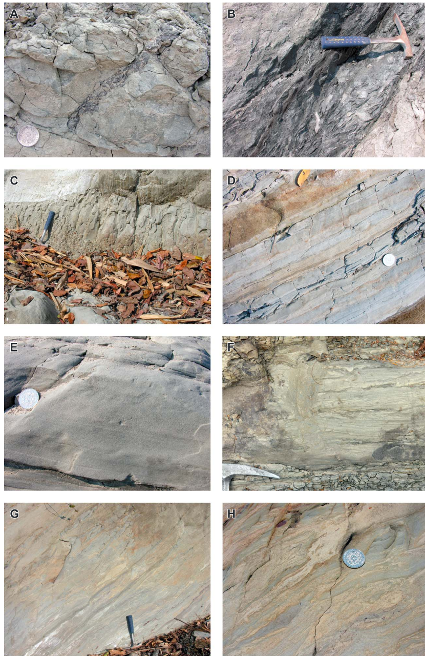
Figure 11. Photographs of outcrops depicting the most typical facies observed in the Dungsam Chu sedimentary section. (a) Facies F1 (units 1 and 2): example of a root trace. (b) Facies F2 (units 1 and 2): carbonaceous shale. (c) Facies F3 (units 1 and 2): noncarbonaceous shale. (d) Facies F4 (units 1 and 2): heterolithics with flat and undulating laminations, some rip-up clasts, and irregular surfaces of the base of the sandstone layers. (e) Facies F5 (units 1 and 2): centimeters to a decimeter thick sequences of normal gradings and flat laminations. (f) Facies 6 (unit 2): a sandstone layer of this heterolithic facies showing flaser beddings, undulating and swaley laminations, and intrabedded gutter casts. Among other burrows, note the decimeter-scale Diplocraterion and the frequent millimeter-scale Planolites . (g and h) Facies 7 (unit 2): sandstone with disturbed laminations, wavy to flaser beddings, soft-sediment deformation structures, and millimeter- to centimeter-scale burrows. (i) Facies 7 (unit 2): sandstone with wavy to flaser beddings and wave ripples. (j) Facies 7 (unit 2): sandstone with flaser beddings, undulating, hummocky, and swaley laminations of wave ripples, and millimeter- to centimeter-scale burrows. (k) Facies 7 (unit 2): sandstone with disturbed laminations, soft-sediment deformation structures, and pervasive bioturbation. (l) Facies 8 (units 1 and 2): sandstone with cross laminations and climbing ripples. (m) Facies 9 (units 1 and 2): sandstone with flat and cross beds, lignite laminations, and soft-sediment deformation structures. (n) Facies 10 (units 1–4): sandstone with climbing-ripple cross-laminations, flat and cross beds, and reactivation surfaces. (o) Facies 11 (units 3 and 4): sandstone with flat and cross beds underlined by scattered pebbles. (p) Facies 12 (unit 4): conglomerate with an erosional basal surface and winnowed gravels at the top.
