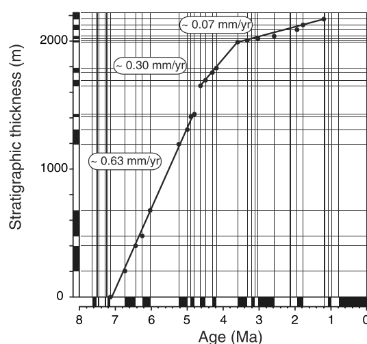
Figure 12. Age versus depth plot of the Dungsam Chu section using the correlation from Figure 9c.
