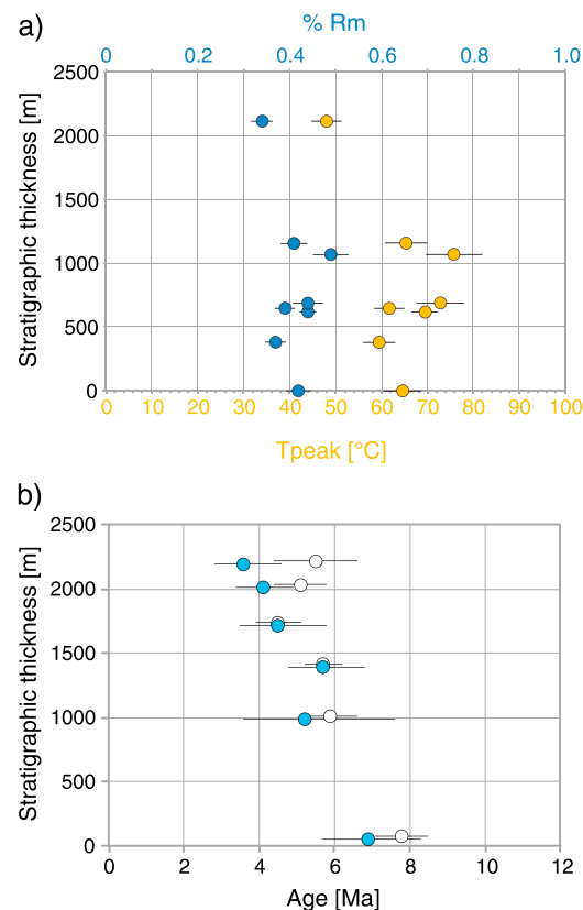
Figure 4. (a) Vitritine reflectance data plotted against stratigraphic depth. In blue are the R_m % and in orange are the peak temperatures calculated according to the calibration of the R_m by Barker and Pawlewicz [1994]. (b) Detrital apatite fission track mean central ages (white circles) and P_1 ages (blue circles) plotted as a function of stratigraphic thickness from the bottom (0 m) to the top (2,216 m) of the section.
