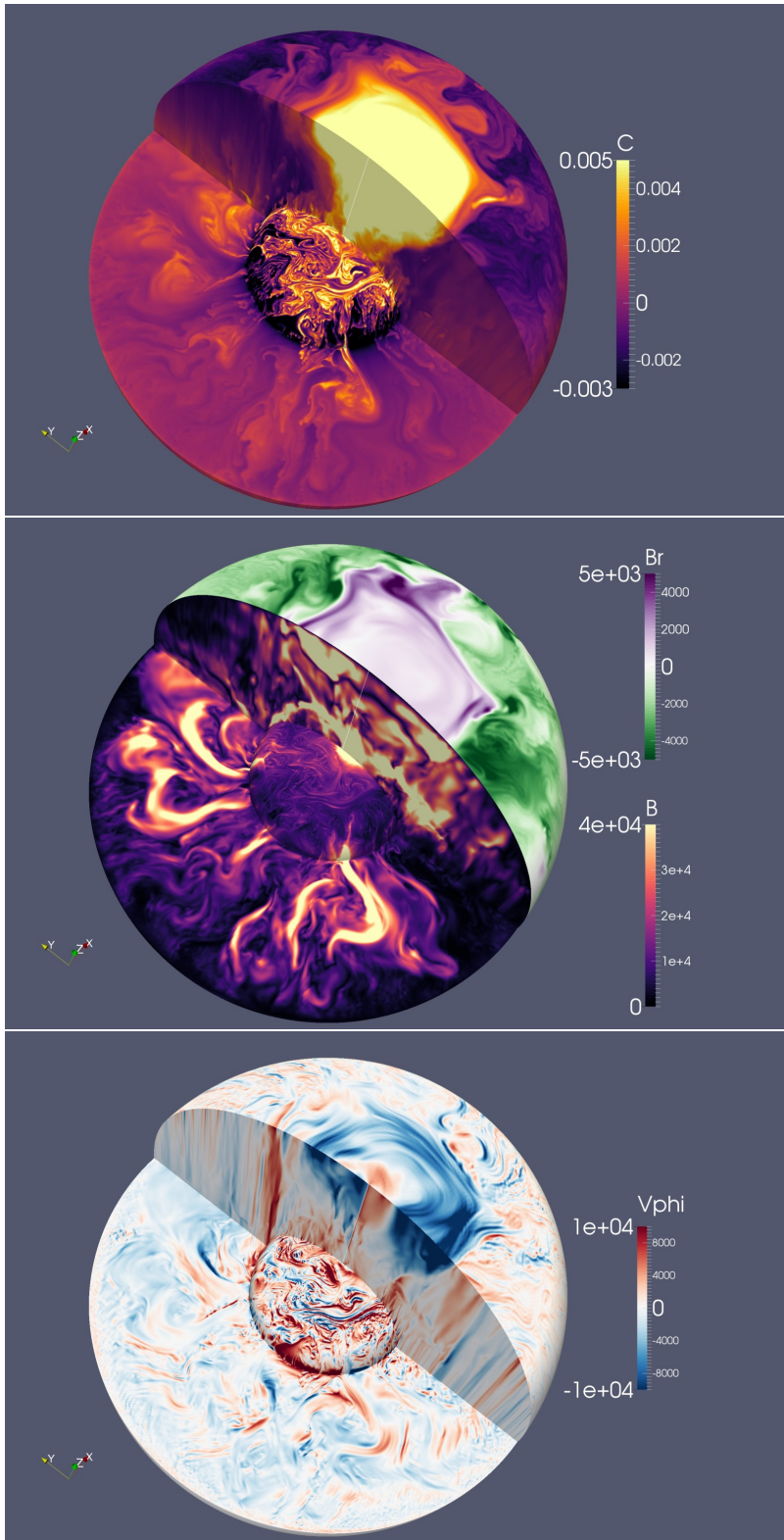
Figure 7: Three-dimensional renderings of the fields in the S2 simulation, at the instant marked by a square in figure 2. The white line is the rotation axis.
