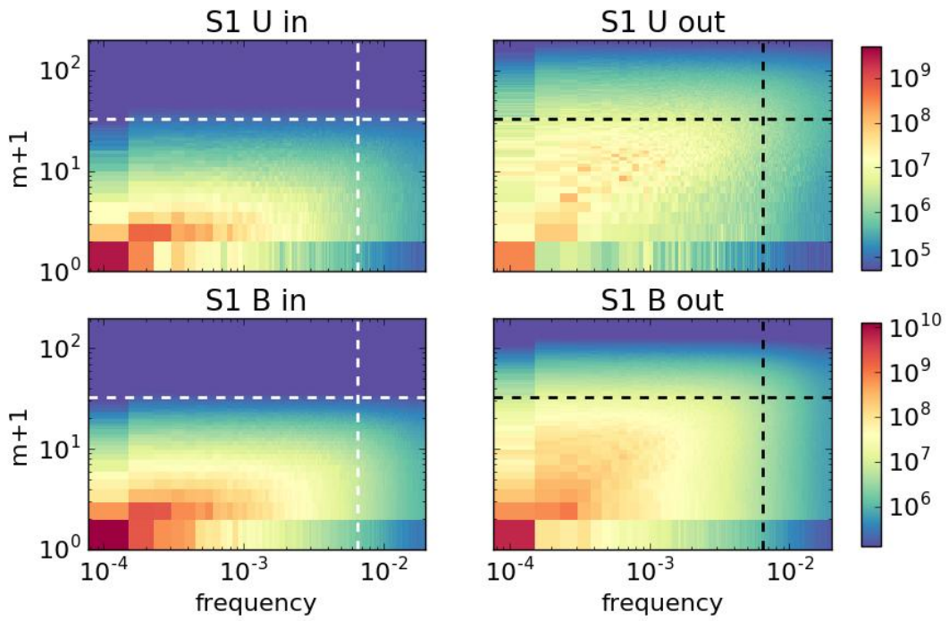
Figure 15: Space-time spectra of the kinetic and magnetic energies in S1. See caption of Fig. 14.
