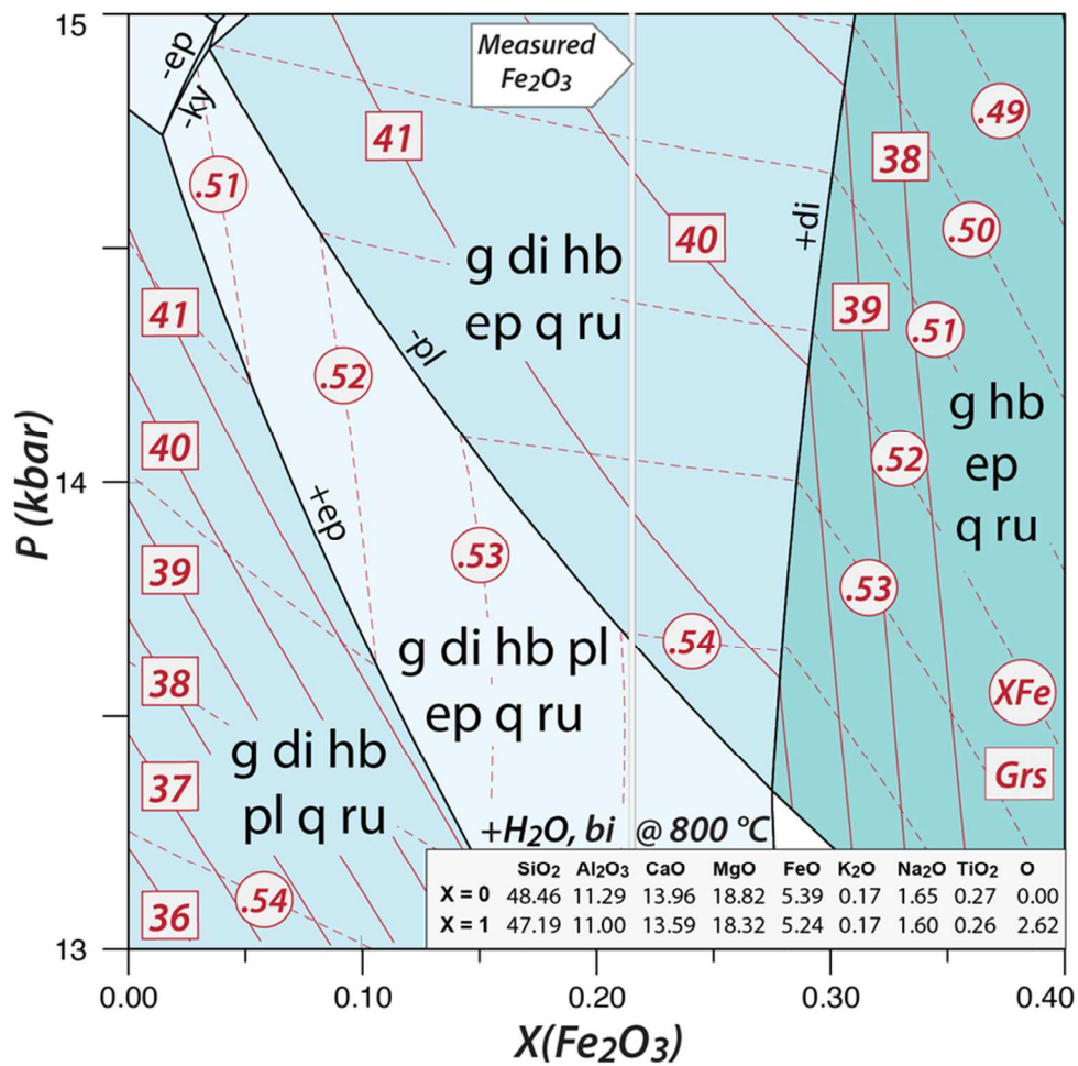
Figure 16: P-X(Fe 2 O 3 ) pseudosection / kyanite-eclogite sample 8023F. – 80mm
