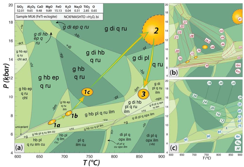
Figure 11: Pseudosection calculated for the Fe-Ti-rich eclogite (MU6). – 170mm 129x88mm (300 x 300 DPI)
