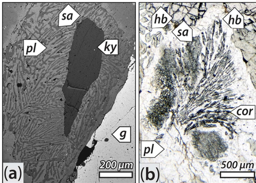
Figure 8: Textures in kyanite eclogite sample 8023F. – 80mm
