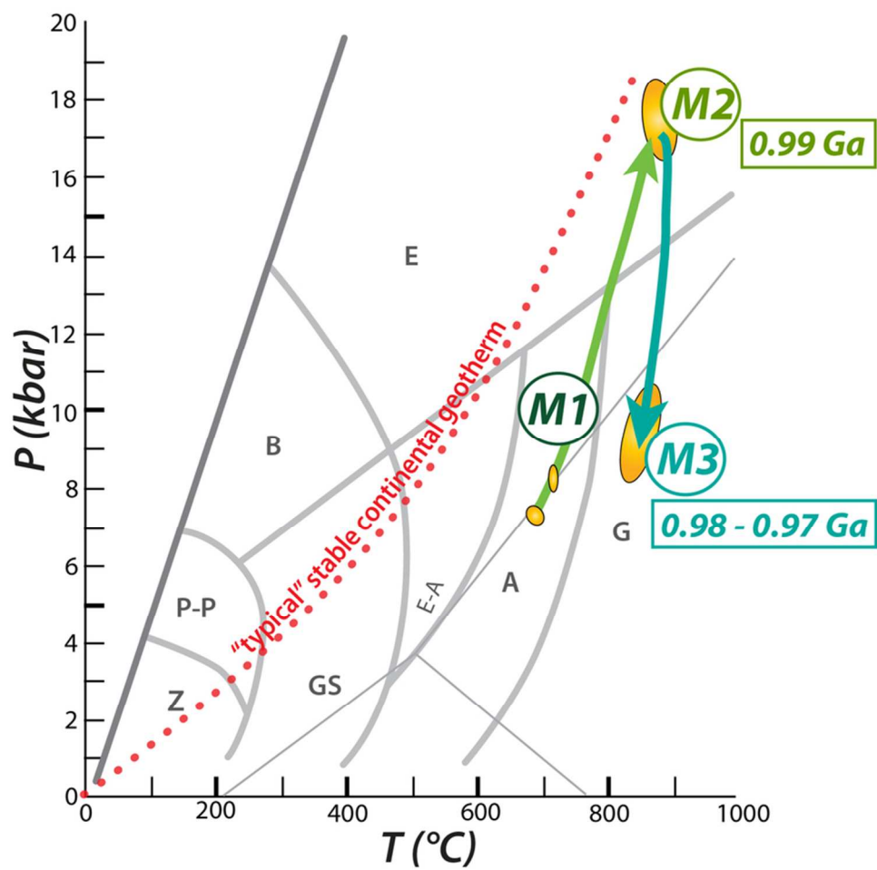
Figure 18: P-T path for Sveconorwegian eclogite, based on the modelling presented in this study. – 80mm
