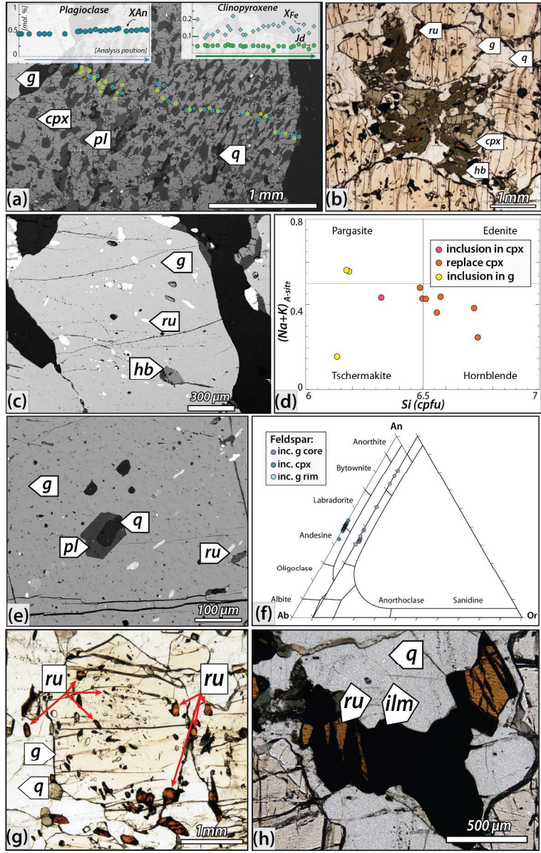
Figure 5: Textures and mineral compositions in Fe-Ti-rich eclogite sample MU6. – 170mm
