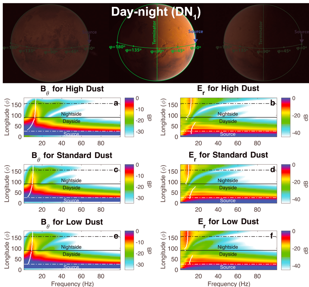
Figure 2. (top) Schematics of the DN_1 simulation. (a, c, and e) Magnetic and (b, d, and f) electric field power spectra as a function of frequency and distance to the source ( \phi ), for the different dust scenarios. The white (black) horizontal dash - dot lines correspond to cuts at \phi = 25^\circ ( \phi = 155^\circ ), used in Figure 4.
