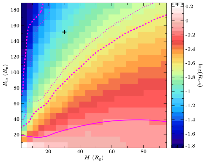
Figure 3. Confidence contours of \chi^2 for the self-consistent relxilllp model as a function of coronal height H and inner radius R_{in} . The lines indicate the 1\sigma (dotted), 90% (dashed), and 99% (solid) confidence levels for two parameters of interest. The 99% level only provides a lower limit to the inner radius. The cross marks the best-fit value. The color-coded map in the background shows the corresponding reflection fraction according to the scale on the right.
