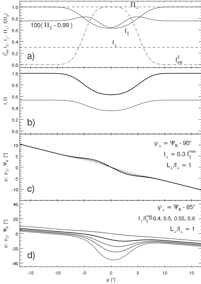
Fig. 14. Influence of the secondary polarisation mode (this time it is the X mode) on the polarisation of a single notch dominated by the primary O mode. A Gaussian void in emissivity \eta_{||} of width \sigma_{\eta} = 2.53^\circ is now applied only for the O-mode emission. The layout is analogous to that of Fig. 7, except in panel d the modes are not precisely orthogonal ( \psi_{\perp} = \psi_B - 85^\circ ). The contribution of the X mode does not much increase the amplitude of the PA wiggle in panel c (cf. Fig. 7c). The slight non-orthogonality of 5^\circ (panel d) transforms the zigzag-shaped wiggle into a one-directional U-shaped distortion of PA (imagine a variant of Fig. 10c with the vector C shorter than A and B). List of parameters: \psi_{||} = -0.6\phi , \rho_{\text{crv}} = 10^4 cm, \nu = 1 GHz.
