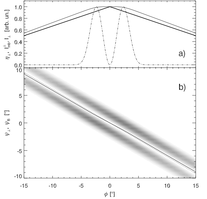
Fig. 16. Polarisation of a very wide emission structure with the triangular emissivity pattern shown in panel a (thick solid line). The net PA (solid line in panel b) nearly follows \psi_B , but not exactly.
