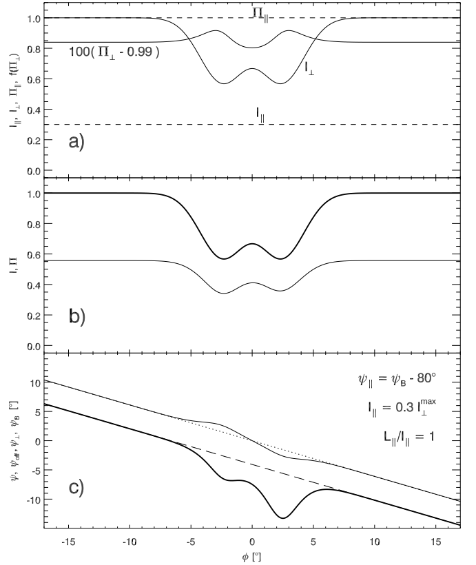
Fig. 9. Polarisation of double notches in the presence of a slightly non-orthogonal secondary polarisation mode ( \psi_{\parallel} = \psi_B - 80^\circ , I_{\parallel} = 0.3 I_{\perp}^{\max} ). The dashed line in c presents \psi_{\text{off}} , i.e. the interpolated off-notch trend of the total PA. The total PA at both minima is located below \psi_{\text{off}} (see the explanation in Fig. 10).
