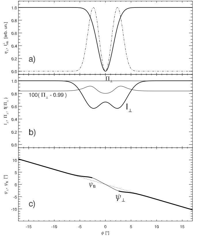
Fig. 6. Result of a calculation which produces the PA wiggle at a nearly merged double notch feature. a) Microbeam intensity I_{\text{mb}}^{\perp} (dot-dashed line) and the macroscopic emissivity with a Gaussian cavity at \phi = 0 (thick solid). b) Net polarisation fraction \Pi_{\perp} (top thin solid) and net X-mode intensity profile (thick solid). The \Pi_{\perp} is slightly smaller than 1, as shown by the bottom thin line presenting the quantity 100(\Pi_{\perp} - 0.99) . c) Net X-mode PA ( \psi_{\perp} , solid) overplotted on the reference \psi_B (dotted). The central part of \psi_{\perp} is thinner to reflect the lack of high-quality data points at the centre of notches in B1821–24A (see Figs. 1d and 2d). The result is for \sigma_{\eta} = 1.53^\circ , \psi_B = -0.6\phi , \rho_{\text{crv}} = 5 \times 10^4 cm, and \nu = 1 GHz.
