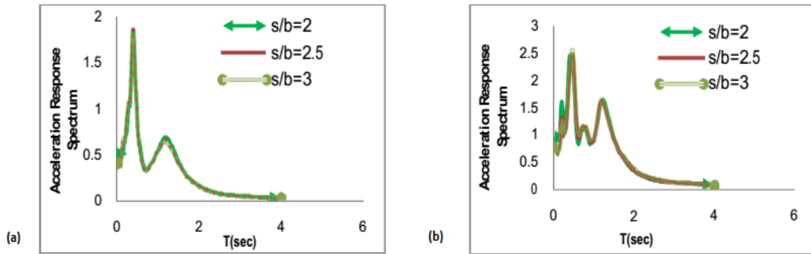
Figure 11. Acceleration response spectra for different pile distance ratios under near-fault Loma Prieta Earthquake with: (a) PGA=0.2g and (b) PGA=0.7g
