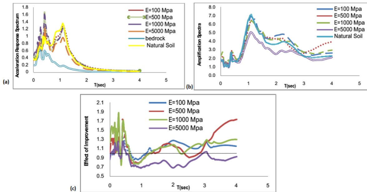
Figure 9. Comparison of seismic response on the surface of the natural ground and its improvement under far-fault Northridge earthquake with PGA=0.2g : (a) elastic response spectra, (b) amplification of S_a , (c) the effect of improvement on S_a .
