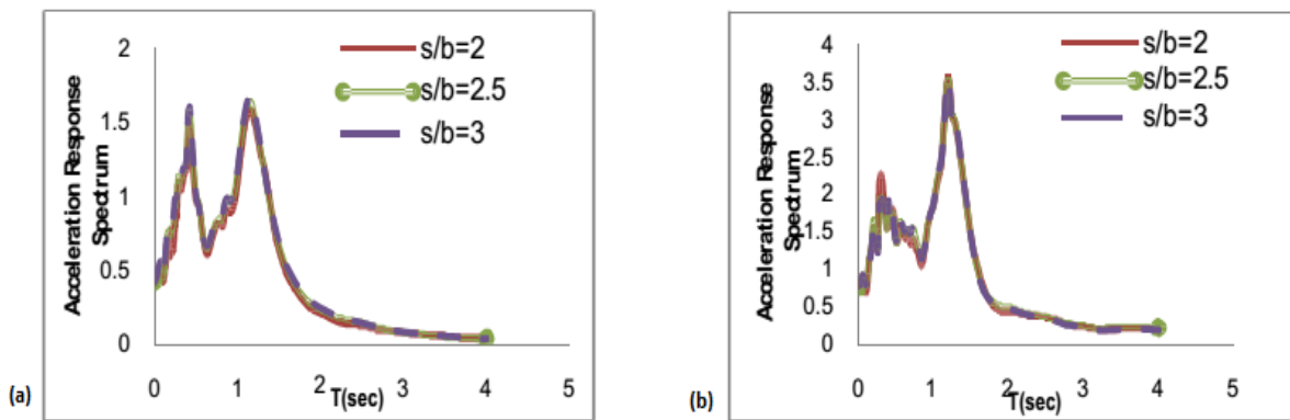
Figure 12. Acceleration response spectra for different pile distance ratios under far-fault Loma Prieta Earthquake with: (a) PGA=0.2g & (b) PGA=0.7g
