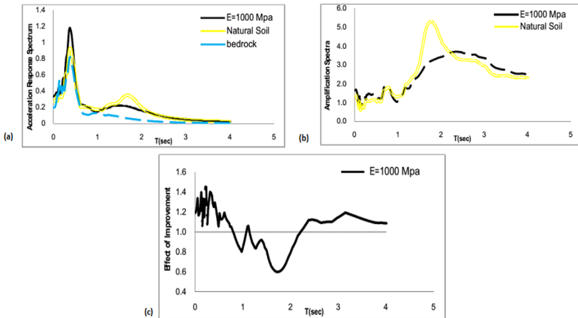
Figure 13. Comparison of seismic response on the surface of the natural ground and its improvement under near-fault Loma Prieta earthquake with PGA=0.2g: (a) elastic response spectra, (b) amplification of S_a , (c) the effect of improvement on S_a
