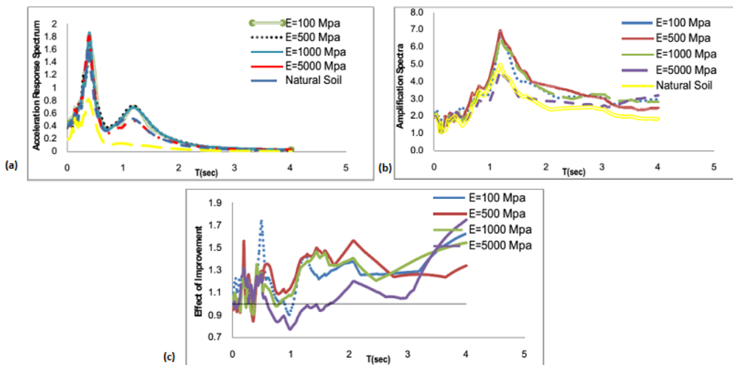
Figure 3. Comparison of seismic response on the surface of the natural ground and its improvement under near-fault Loma Prieta earthquake with PGA=0.2g : (a) elastic response spectra, (b) amplification of S_a , (c) the effect of improvement on S_a
