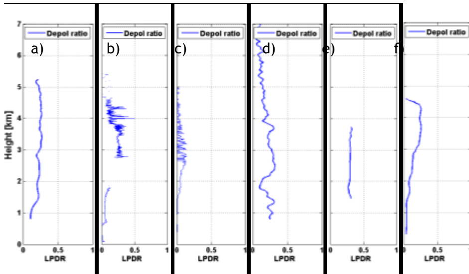
Figure 8. Particle depolarization ratios retrieved by lidar measurements. From the left to the right the stations are Granada at 532 nm (a), Cap d'en Font at 355 nm (b), Ersa at 355 nm (c), Naples at 532 nm (d), Potenza at 532 nm (e), Lecce at 355 nm (f). The date of the measurements are 17 June at 01 UTC, 18 June at 12 UTC, 20 June at 15 UTC, 22 June at 10:46 UTC, 21 June at 23:40 and 22 June at 11:18 for Granada, Cap d'en Font, Ersa, Naples, Potenza and Lecce respectively. The bottom and top heights are 2236 and 5994 m in Granada, 201 and 5787 m in Cap d'en Font, 1360 and 4848 m in Ersa, 1768 and 7468 m in Naples, 1630 and 5530 m in Potenza and 1484 and 5081 m in Lecce.
