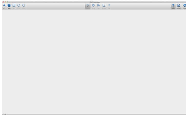
Figure 3.1 – ChronoModel interface
