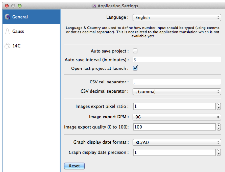
Figure 3.7 – Application settings
