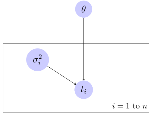
Figure 2.1 – DAG representation of the Event model. Directed edges represent stochastic relationships between two variables, blue circles represent unknown parameters. Rectangular plates are used to show repeated conditionally independent parameters.
