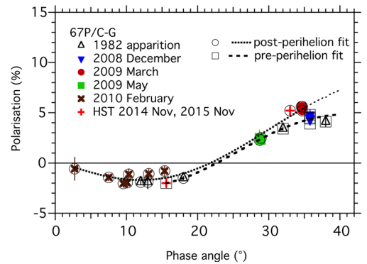
Figure 5 Linear polarization data as a function of phase angle for 67P/C-G. Data from Myers & Nordsieck 1984 (1982 observations); Hadamcik et al. 2010 (2008–2009 observations); Stinson et al. 2016 (2010 observations); Hines & Levasseur-Regourd 2016 (2014 observations); this work for HST in 2015 November at a 33^\circ phase angle. A difference between the two phase curves, fitted for data before and after perihelion, is visible at least for phase angles above 30^\circ . Some error bars are smaller than the signs. The errors are taken into account in the two fits. Red-wavelength domain.
