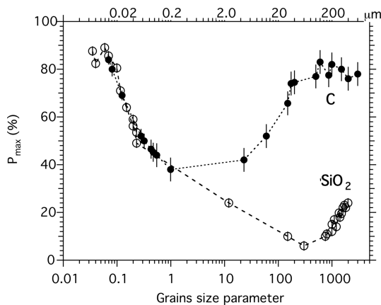
Figure 11. Polarization value versus size parameter X of the grains ( X = 2\mu s/\lambda , where s is the equivalent radius and \lambda is the wavelength of measurements). C, carbon black; \text{SiO}_2 , silica. (Updated from Hadamcik et al. 2009.)
