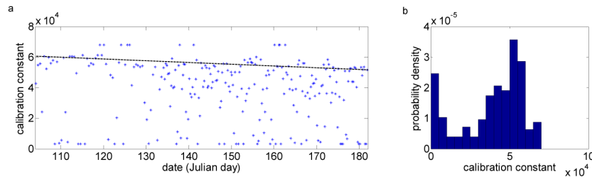
Fig. 4. a) System constants calculated for profiles from the first period of Barneo campaign, including icing correction. The line of points at the bottom represents measurements with a limited correction factor ( N-IcI < 0.05 ). These points are removed in the analysis but kept in the probability density figure to show their distribution. b) Probability density function of system constants for the first period of the Barneo campaign. The peak on the left corresponds to the limitation of the correction factor. The dashed line corresponds to a fit of the maximum calibration values excepting the few clear window values.
