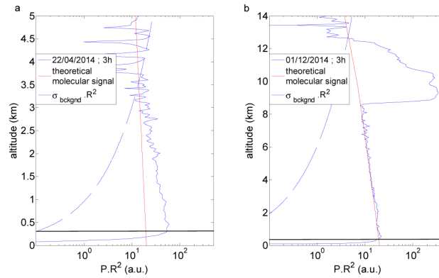
Fig. 2. Daytime (left) and nighttime (right) range corrected signals obtained after deployment of the buoy at Barneo in April 2014 (IAOOS 2). Solid black line is indicative of the overlap range.
