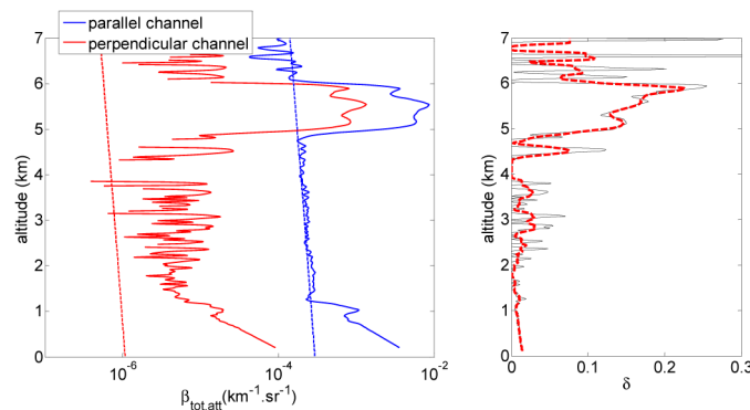
Fig. 7. left: total attenuated backscatter coefficient measured in both co- and cross-polarizations during the N-ICE2015 campaign (IAOOS 6), assuming a similar system constant, with theoretical normalized molecular signal as dashed lines (assuming a 0.36% depolarization for the red), and right: depolarization ratio obtained with calibration by polarization rotation method, and with convolution over 200m for the red dashed curve. See text for discussion of uncertainties and biases.
