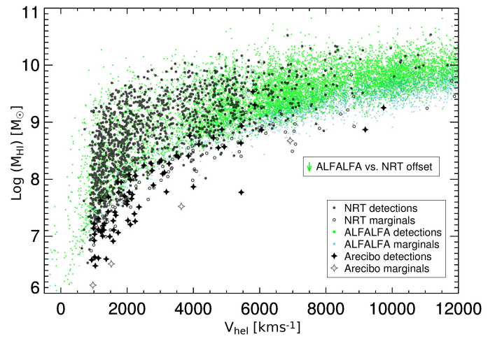
Fig. 8. Total HI mass, M_{\text{HI}} (in M_\odot ), as a function of HI radial velocity (in \text{km s}^{-1} ). Shown are the NIBLES detections and marginals from both our Arecibo and Nançay observations (black stars and dots respectively), together with data based on the ALFALFA \alpha.40 catalog (Haynes et al. 2011), where green dots represent detections (their Category 1) and light blue dots represent marginals (Category 2). Excluded were all NIBLES detections which are definitely or probably confused by another galaxy within the telescope beam, as well as detections that are likely resolved (see Paper I). The HI masses of the ALFALFA detections were calculated in the same way as for the NIBLES sources, using simply a distance of D = V/H_0 , where the adopted Hubble constant is H_0 = 70 \text{ km s}^{-1} \text{ Mpc}^{-1} . The green vertical arrow above the legend indicates the difference of 0.16 in \log(M_{\text{HI}}) corresponding to the mean HI flux scale difference between the \alpha.40 catalog and our NRT data.
