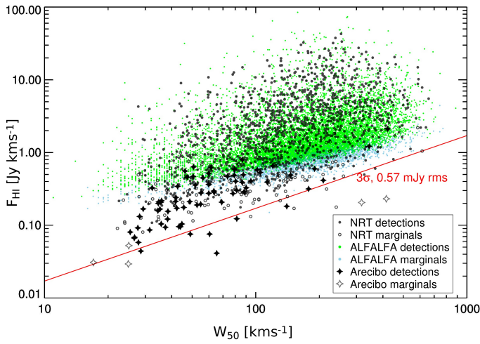
Fig. 7. Integrated HI line flux F_{\text{HI}} (in \text{Jy km s}^{-1} ) as a function of W_{50} line width (in \text{km s}^{-1} ). Shown are the NIBLES non-confused and non-resolved detections and marginals from both our Arecibo and Nançay observations, together with the ALFALFA data from the \alpha.40 catalog (Haynes et al. 2011), where green dots represent detections (their Category 1) and light blue dots represent marginals (Category 2). The red line indicates the integrated line flux from a 3\sigma flat-topped profile with a 0.57 mJy rms noise level.
