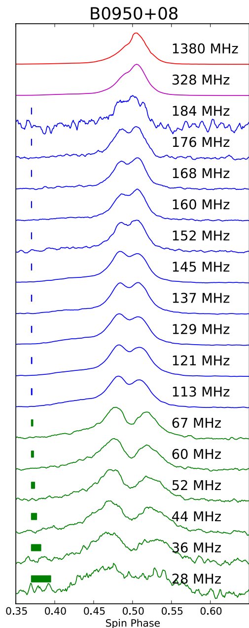
Fig. 1. Example of pulsar profile evolution for PSR B0950+08, from 1400 MHz down to 30 MHz. It becomes more rapid at low frequencies. The bars on the left represent the intra-channel smearing due to uncorrected DM delay within a channel at each frequency. The profiles were aligned using a timing ephemeris (see text for details).
