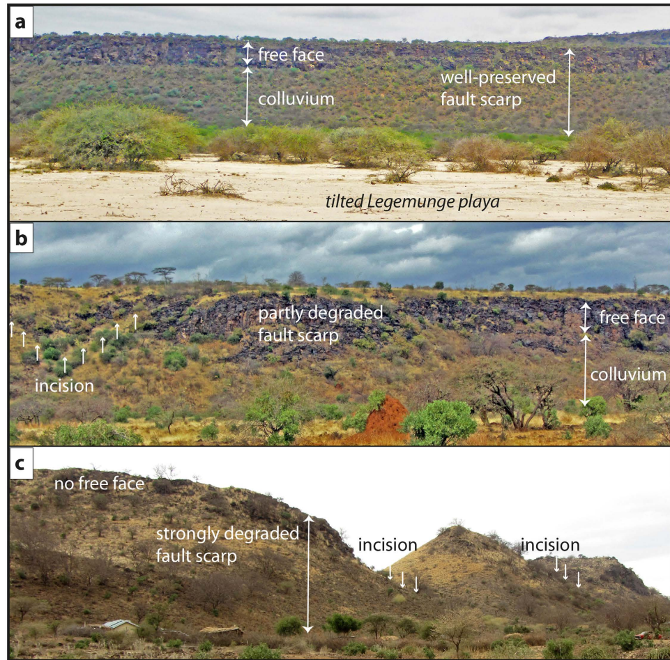
Figure 2. Fault scarps in trachyte of the Olorgesailie region displaying different stages of degradation.
