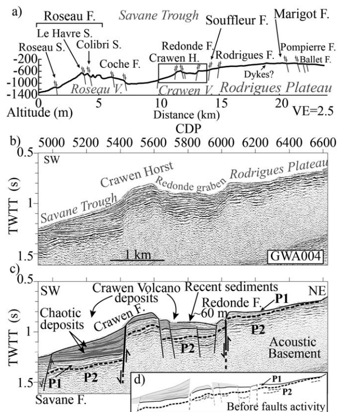
Figure 10. Interaction between faults and Crawven volcano deposits. (a) Bathymetric profile, located in Figure 2a by white brackets. (b) Data and (c) interpretation of the 72 channel seismic profile GWA004, located in Figure 2b by a white dashed line. (d) Reconstruction of the profile before faulting. Using a uniform wave propagation velocity of 1800 m/s in the sediments [Shalev et al. , 2010], the faults would dip by about 65°–80° northeastward.
