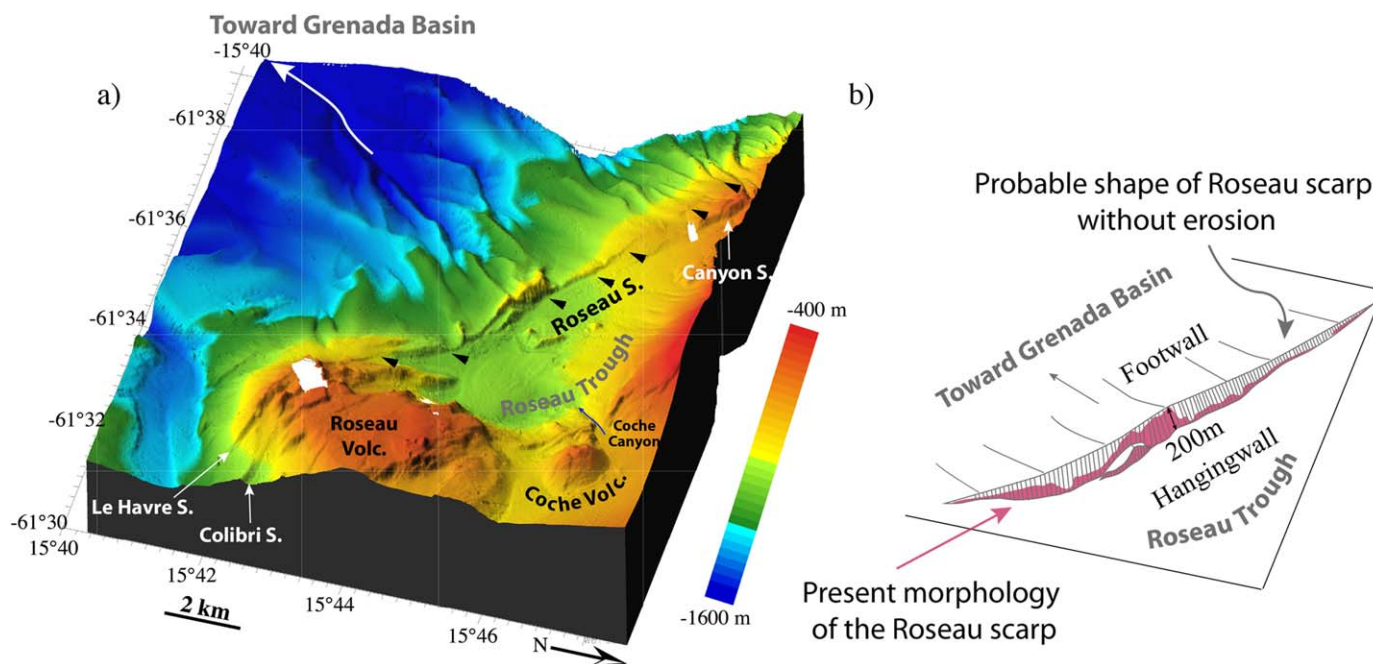
Figure 13. The Roseau fault footwall is eroded by retrogressive erosion, which induces high fluctuations in its scarp height when canyons reached the scarp edge. (a) 3-D view of the area. (b) Morphology of the Roseau scarp: present morphology in pink compared to a probable scarp shape in grey that would not have suffered from erosion.
