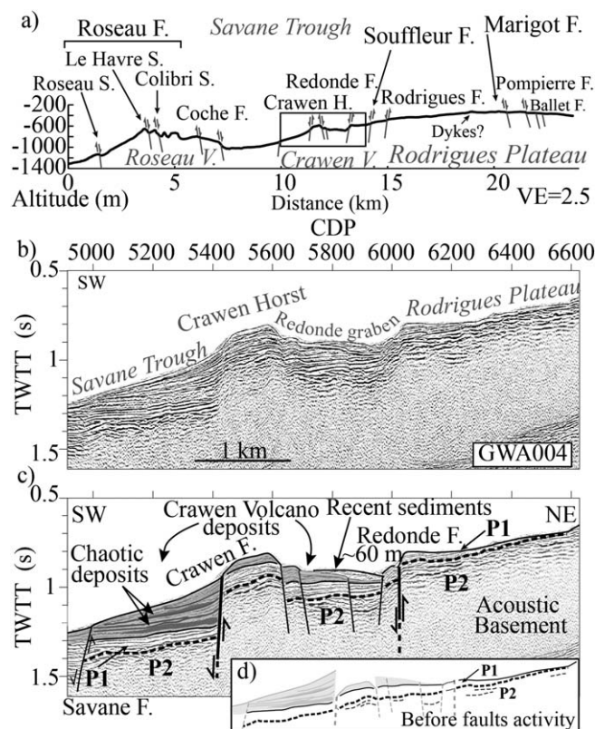
Figure 10. Interaction between faults and Crawlen volcano deposits. (a) Bathymetric profile, located in Figure 2a by white brackets. (b) Data and (c) interpretation of the 72 channel seismic profile GWA004, located in Figure 2b by a white dashed line. (d) Reconstruction of the profile before faulting. Using a uniform wave propagation velocity of 1800 m/s in the sediments [Shalev et al., 2010], the faults would dip by about 65°–80° northeastward.
