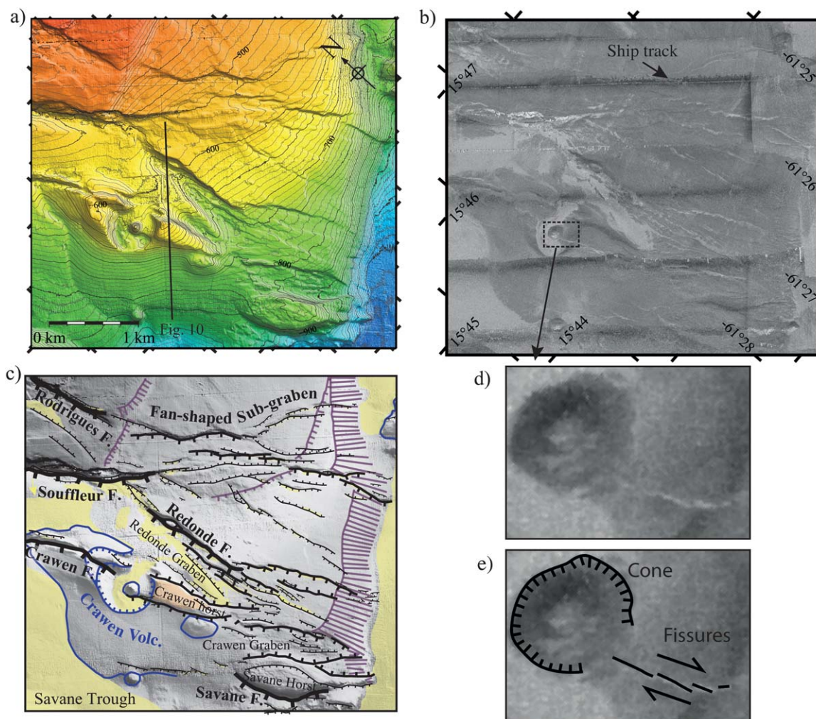
Figure 7. The southern tip of Rodrigues, Souffleur, and Redonde faults fan out southward in a damage zone and interact with the Crawen volcano. (a) Bathymetric map, isobaths every 10 m, main lines every 50 m. (b) Backscatter image of the area, the darker the more reflective. Fault-bounded basin appears in light grey, probably due to the presence of fine-grained sediments. (c) Detailed fault map of the area, in black, thicker traces for higher scarps. Crawen volcano in purple. Rodrigues plateau's escarpments in dark red lines. (d) Close-up view of Crawen volcano dome at the tip a left-stepping fissures and (e) map of the fissures.
