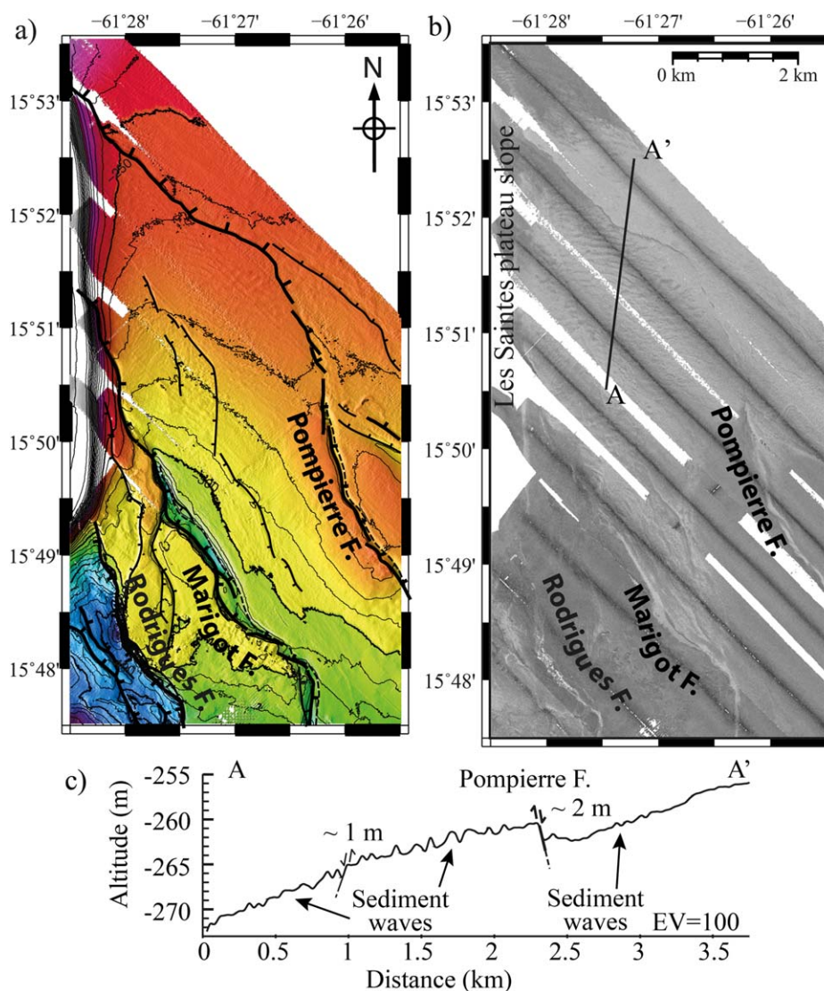
Figure 14. Marigot and Pompiere faults are crosscutting sediment waves at the base of Les Saintes plateau: (a) bathymetry, (b) backscatter image, location in Figure 2b. (c) Bathymetry profile AA'. The sediment waves are ~1 m high and tens meters wide and offset by 2–5 m.
