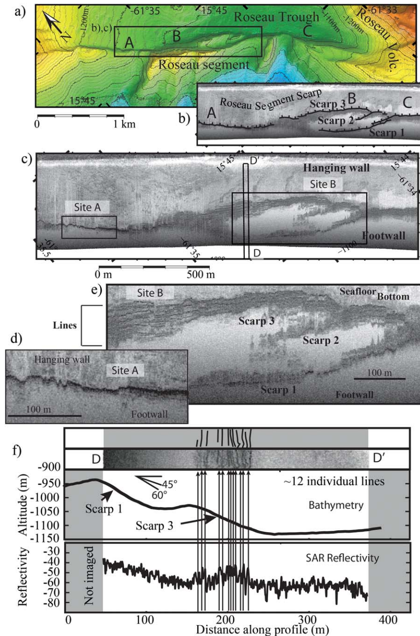
Figure 4. Details of Roseau segment escarpment, located in Figure 2b. (a) Bathymetry of the Roseau segment, isobaths every 20 m; (b) detailed fault map of the Roseau segment on the SAR image enlarged in Figure 4c, the darker the more reflective. (d, e) Close-up of the SAR image on sites A and B. (f) Comparison between SAR image: (top) interpretation and data, (middle) bathymetry, and (bottom) SAR reflectivity along DD' profile perpendicular to the scarp. Black and white alternations creating lines identified in the SAR image, correlated to bathymetry and reflectivity by black arrows. As the SAR is a deep-towed acoustic system driven at few tens of meters above the seafloor, the highest part of the scarp is not imaged (grey area).
