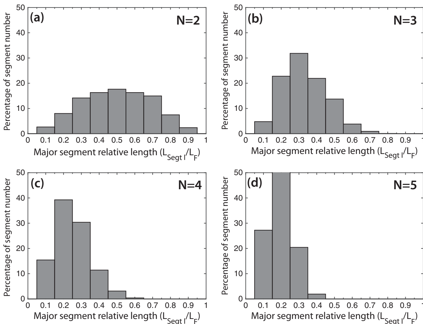
Figure 8. Distribution of the major segment lengths ( L_{Seg I} ) relative to their master fault lengths ( L_F ), for faults discriminated by their number N of major segments. (a–d) Faults having 2, 3, 4, and 5 major segments, respectively.
