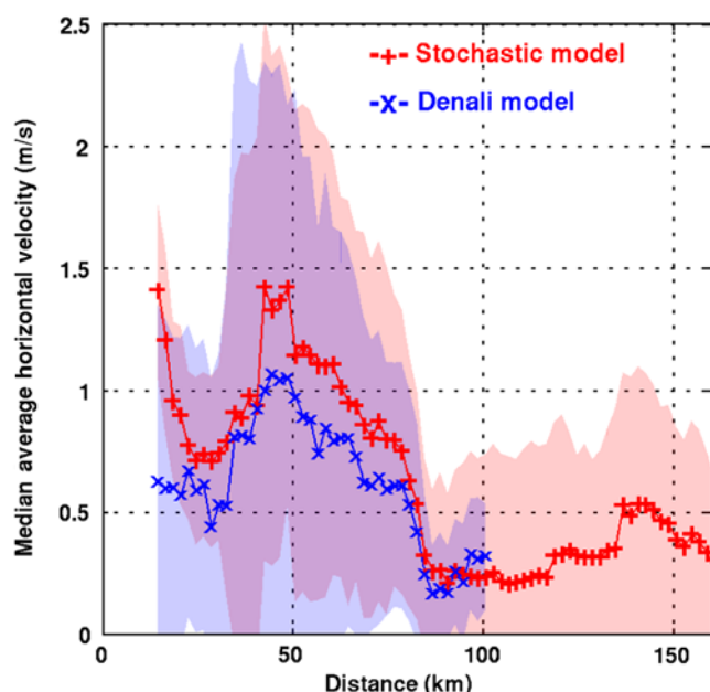
Figure 24. Median peak average horizontal velocity (m/s) (+, stochastic model; x, the Denali model) as a function of source-to-site distance, in southern California due to an M_w 7.9 earthquake occurring along the southern San Andreas fault. The shaded region corresponds to median \pm 1 standard deviation. A total of 10 rupture scenarios (five rupture locations \times two propagation directivity) are considered.) The color version of this figure is available only in the electronic edition.
