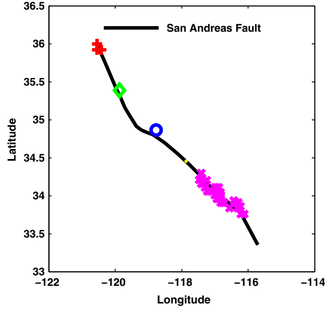
Figure 8. Locations along the southern San Andreas fault at which stress estimates are available from the World Stress Map project. Five data clusters are shown (plus-, diamond-, circle-, dot-, and cross-marked points). The color version of this figure is available only in the electronic edition.
