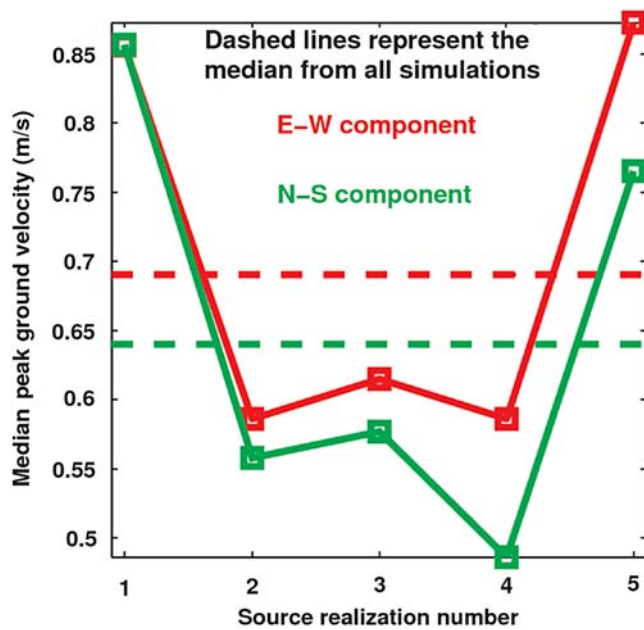
Figure 16. The solid lines are median peak ground velocity (PGV) computed at 636 sites in southern California from 10 rupture scenarios (five rupture locations along the southern San Andreas fault \times two rupture directions) using each of five stochastic source realizations. The dashed lines are the corresponding median PGV from all 50 scenario earthquakes. All earthquakes are of magnitude M_w 7.9. (E-W, east–west component; N-S, north–south component.) The color version of this figure is available only in the electronic edition.
