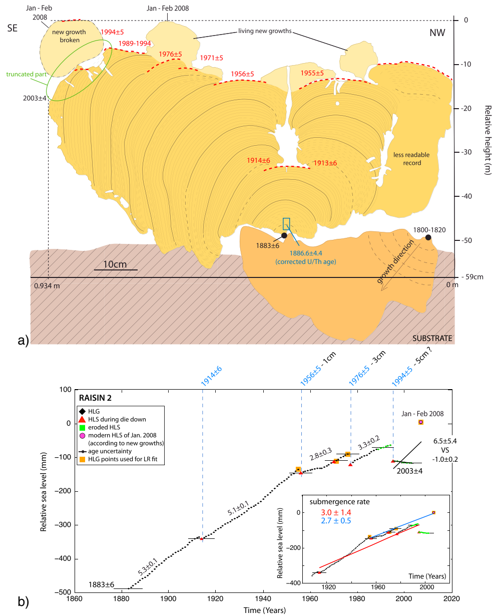
Figure 10. Slab stratigraphy of Raisin 2. (a) Symbols and dates as in Figure 5. The coral base detached from the main slab is drawn in orange but was not X-rayed. Growth band counting on that part was based on growth rate of the species and growth band counting of the top (X-rayed) part. Blue rectangle: U/Th sample location with date and uncertainty (Table 1). (b) HLS curve of Raisin 2. Symbols, rates, and dates as in Figure 5. For the blue straight line, we have considered that the modern HLS outlined by new growths in 2008 is the last HLG (see Text S4 in the supporting information).
