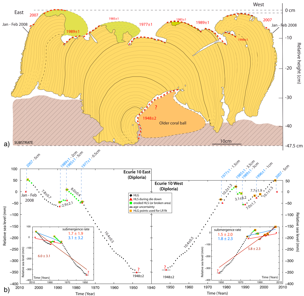
Figure 11. Slab stratigraphy of Ecurie 10. (a) Symbols and dates as in Figure 5. Green area: as in Figure 8a. The older coral on which Ecurie 10 began to grow is drawn in orange. (b) HLS curve of Ecurie 10. Symbols, rates, and dates as in Figure 5. The HLS curves have been constructed for each radius and positioned relative to each other. Inset: brown straight lines: submergence rate treating 1948 ± 2 as the first HLS (see Text S4 in the supporting information).
