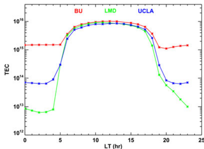
Figure 5. The diurnal patterns of total electron content ( \text{e}^-/\text{m}^2 ) from three models run for conditions of 21 April 2015. The Boston University (BU); University of California, Los Angeles (UCLA); and the Laboratoire de Météorologie Dynamique (LMD).
