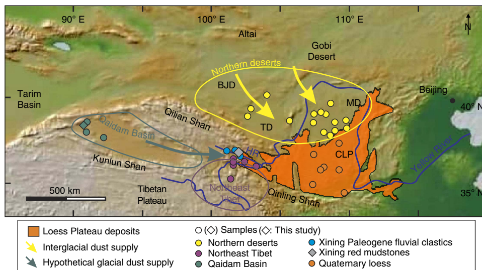
Figure 2 | Dust supply patterns to the Chinese Loess Plateau. The figure shows the modern, simplified dust-storm tracks (yellow arrows), throughout the Mu Us (MD), Tengger (TD) and Badan Jaran (BDJ) deserts, the hypothetical ‘glacial’ dust-storm track (green arrows), throughout the Qaidam Basin 10 , the provenance regions for the Eocene dust (coloured ellipses) and the samples used in this study (description, location and references are provided in Supplementary Data 1). HR, Huangshui River, tributary of the Yellow River (both shown by blue lines) incising the Xining Basin.
