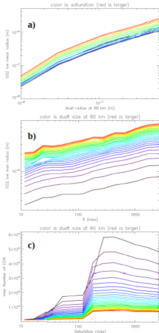
Fig. 3 : Variations of the CO 2 ice particle mean (a), maximum (b) radius and maximum concentration (c) as a function of saturation ratio S and aerosol particle size in the mesosphere.
