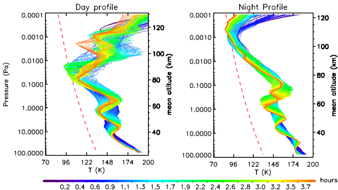
Fig. 1 : Atmospheric temperature profiles with gravity-wave induced cold pockets simulated by the LMD Mesoscale model (Spiga and Forget, 2009 ; Spiga et al., 2012). The red dotted line is the CO 2 saturation curve. From Listowski et al., (2014)
