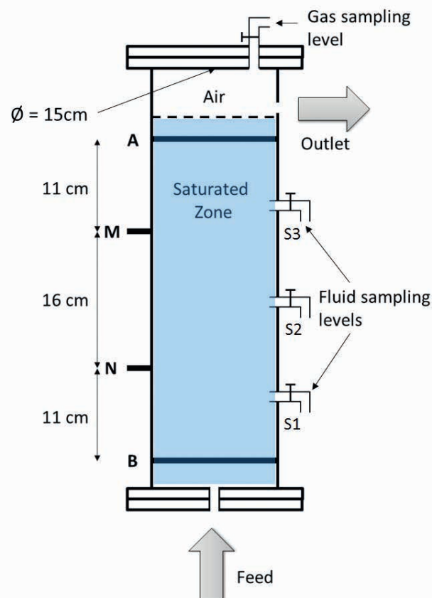
Figure 1 Column design. (Left) SIP measurements disposal: A and B are MP35N ring current electrodes; M and N are handcraft \text{Cu}/\text{CuSO}_4 point potential electrodes. (Right) Gas sampling point at the top of the column, fluid sampling points at three different heights. The column is fed up with bacterial growth medium and toluene.
