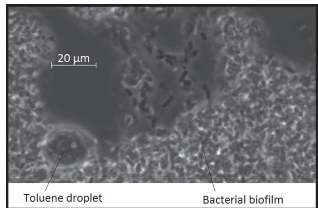
Figure 3 Optical microscope photograph of the biofilm detached from the sand at the top of the inoculated column (day 22). Biofilm seems to include a toluene droplet.
