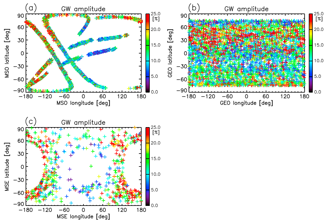
Figure 6. Longitudinal-latitudinal distributions of the GW amplitudes in the (a) MSO, (b) GEO, and (c) MSE coordinates.
