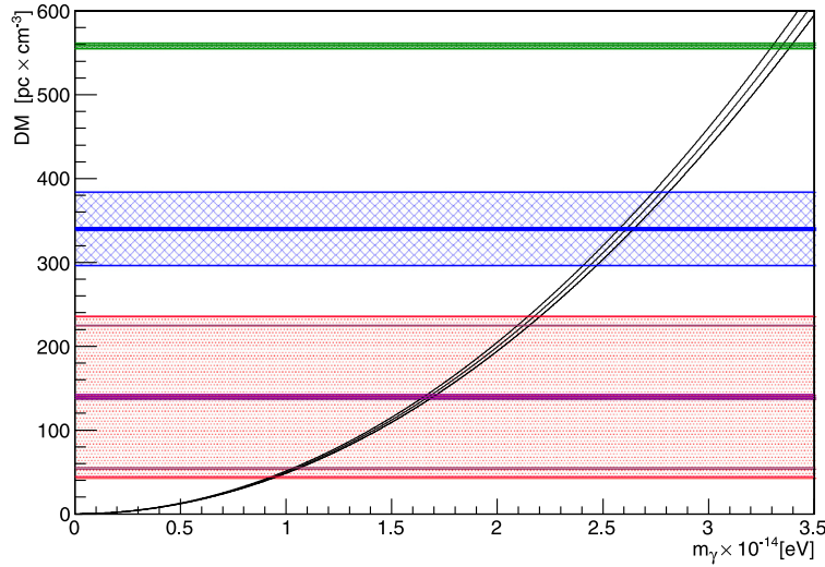
Fig. 1. Contributions to the dispersion measure (DM) budget for FRB 121102. The top (green) band represents the experimental measurement of the total DM = 558.1 \pm 3.3 pccm ^{-3} . The middle (blue) band shows the extragalactic contribution, as obtained by subtracting from the central value of the total DM the galactic contribution DM_{MW} \equiv DM_{NE2001} + DM_{halo} = 218 pccm ^{-3} [23], to which is assigned an estimated uncertainty of 20%. The bottom (pink) band is obtained by subtracting also the estimated contribution from the intergalactic medium (IGM): DM_{IGM} \simeq 200 pccm ^{-3} [23], which has an uncertainty of 85 pccm ^{-3} associated with inhomogeneities in the IGM, and a smaller uncertainty associated with the cosmological parameters (indicated by the narrow magenta band). The outer pink band shows the total uncertainty in the residual DM after subtraction of DM_{MW} and DM_{IGM} , with errors added in quadrature. The curved (black) band shows the possible contribution of a non-zero photon mass, m_\gamma , also including the uncertainties in cosmological parameters and the redshift of FRB 121102. (For interpretation of the references to colour in this figure legend, the reader is referred to the web version of this article.)
