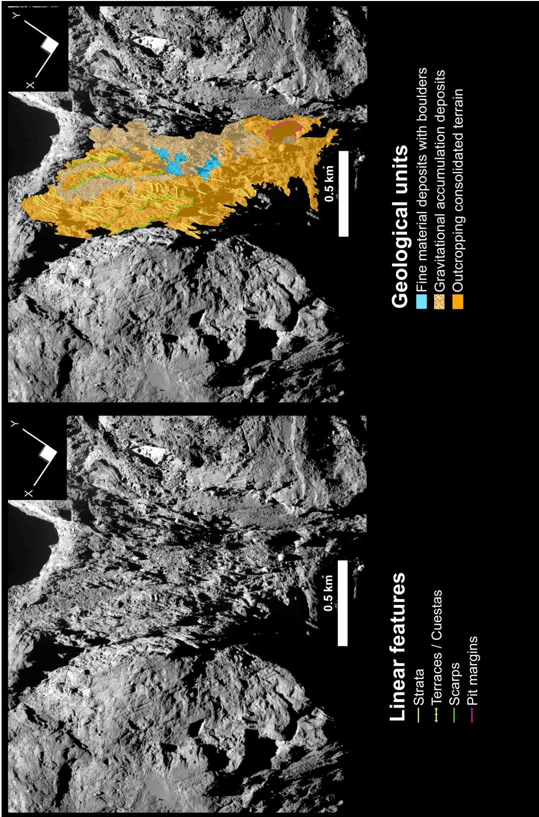
Figure 14. Geomorphological map of Neith and Sobek regions.
