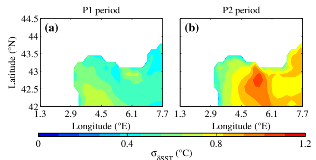
Fig. 7 Standard deviation of the CPL–CTL SST difference \sigma_{\delta\text{SST}} over P1 (a) and P2 (b) periods
