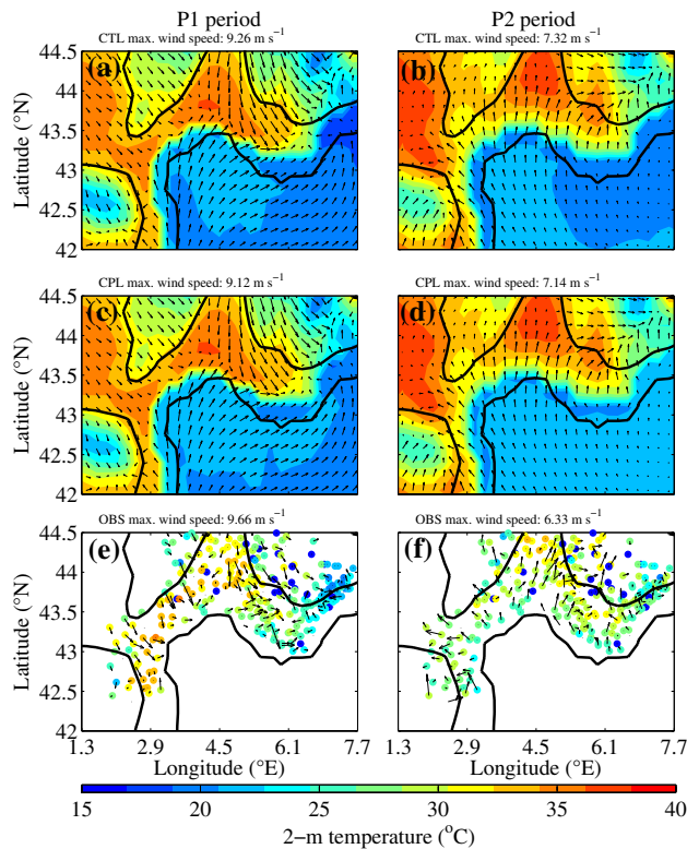
Fig. 2 2-m temperature (color) and 10-m wind (arrows) field averaged over the P1 period (21–23 June 2001) (left column; a , c , e ) and the P2 period (24–26 June 2001) (right column; b , d , f ) at 1800 UTC from CTL (upper row, a , b ) and CPL (middle row, c , d ) simulations, and from the Météo-France surface weather stations measurements (lower row, e , f ). The thick lines indicate the coastline and the 500-m height topography
