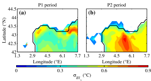
Fig. 12 Significant standard deviation of the CPL–CTL 2-m temperature difference during the P1 period (a) and the P2 period (b)
