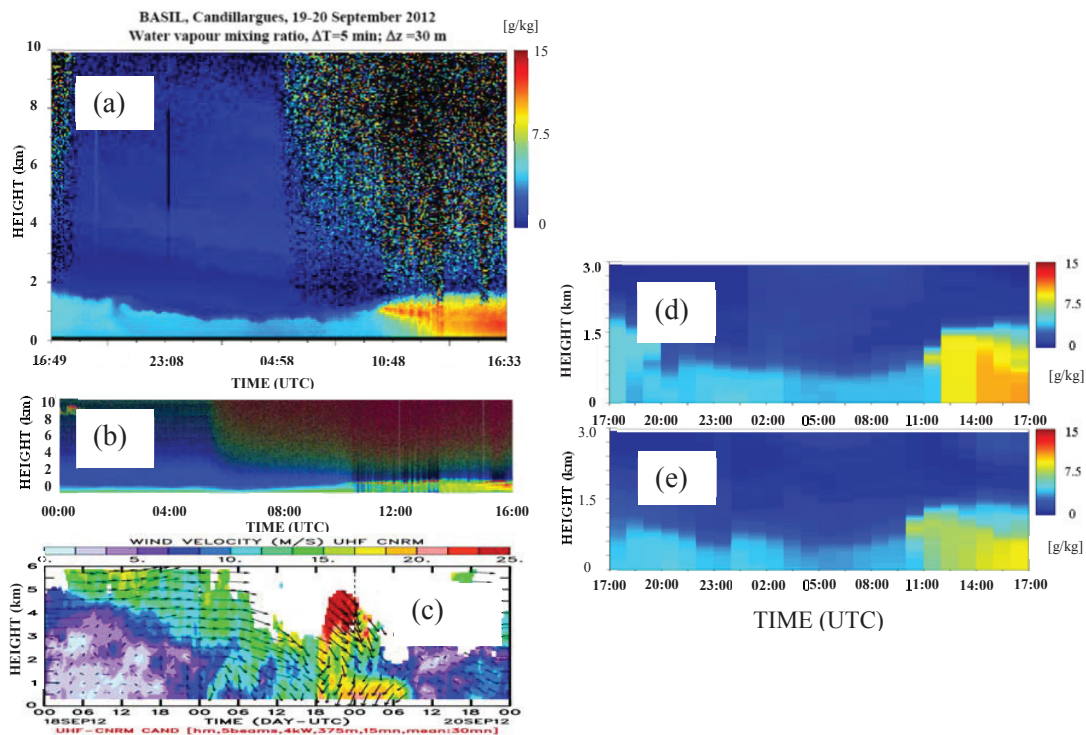
FIGURE 2. a) Water vapour mixing ratio as measured by BASIL over a the time period from 16:49 UT on 19 September 2012 to 16:33 UT on 20 September 2012. b) RCS_{532} as measured by BASIL over the time period from 00:00 UT to 16:00 UT on 20 September 2012. c) Wind speed and directions on 18-19-20 September 2012 as measured by the UHF wind profiler located in Candillargues. e) Water vapour mixing ratio as simulated by the mesoscale models AROME WMED (panel d) and MESO-NH (panel e) over the 24 h time period from 16:00 UT (17:00 UT for AROME WMED) on 19 September 2012 to 16:00 UT (17:00 UT for AROME WMED) on 20 September 2012.
