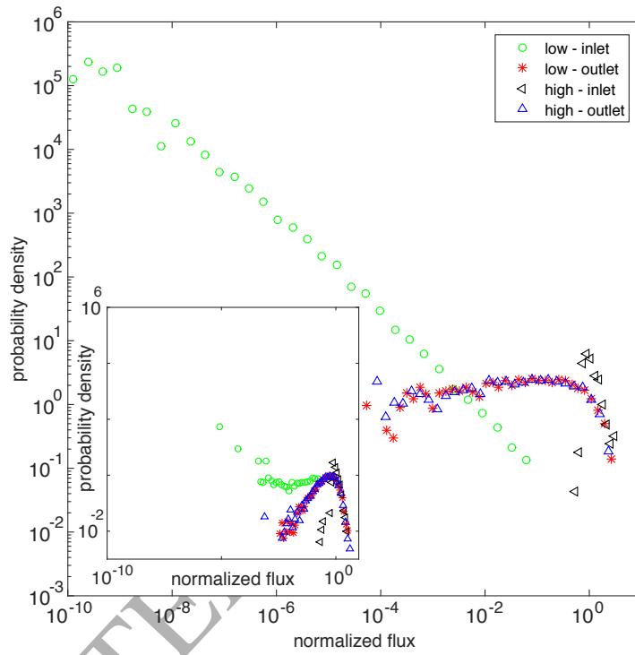
Figure 14: Lagrangian flux distributions at the inlet and outlet with two arbitrary initial velocity distributions for \sigma_{\ln K} = 5 . The two initial velocity distributions come from uniform injections into regions of the 20-percentile highest, and 20-percentile lowest velocities. Flux values are normalized with the mean flux value. Note that flux distributions at outlet are identical regardless of the initial velocity distribution. Inset: same plot for \sigma_{\ln K} = 1 .
