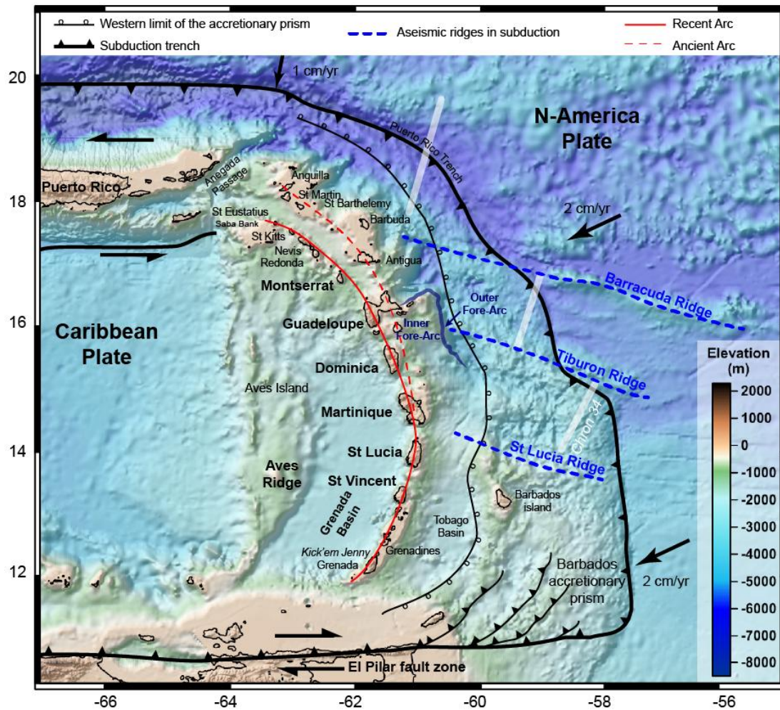
Large scale context of the LAA (after [Bouysse and Westercamp, 1988]).
