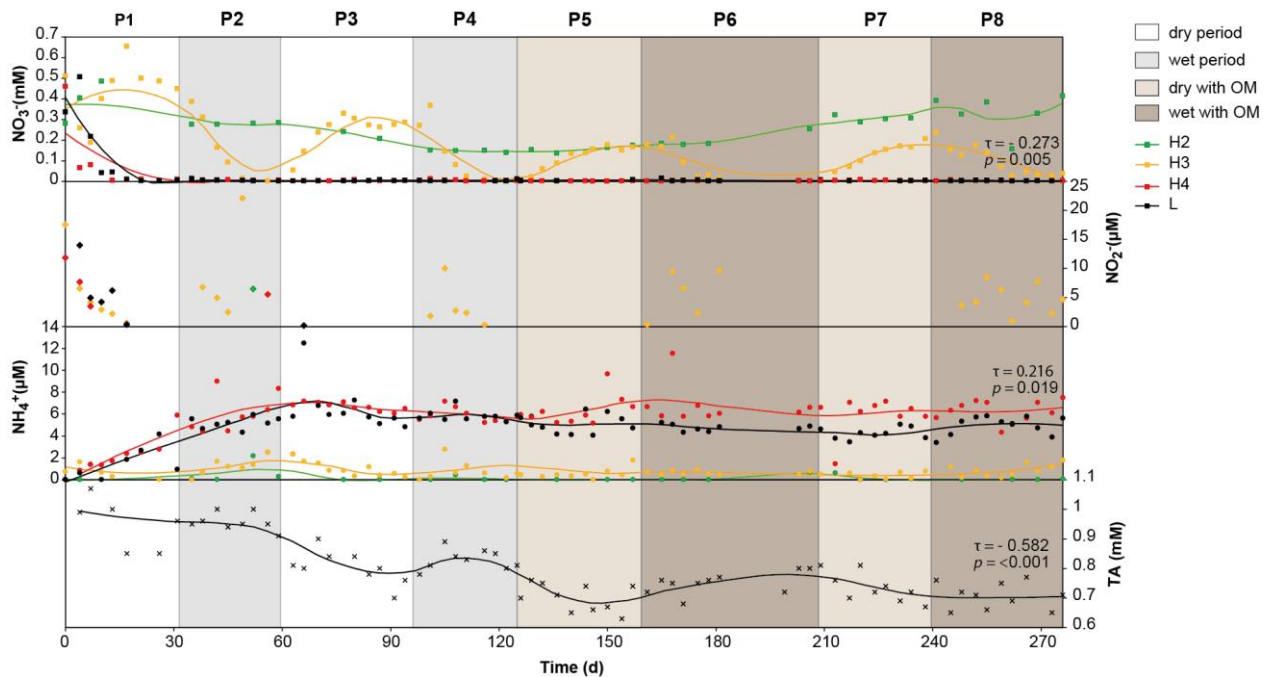
7 Figure 3: Measured evolution of \text{NO}_3^- (square), \text{NO}_2^- (diamond), \text{NH}_4^+ (circle) and TA (cross) concentrations. Curves correspond to smooth local regression (span = 0.3). Kendall's tau ( \tau ) and p -value were given for significant trends with SK test ( p < 0.05 ).
