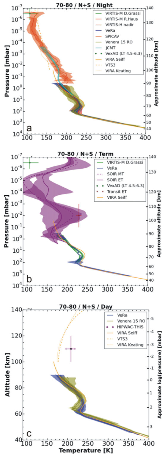
21 Figure 18: same as Figure 15 but for combined temperature profiles from the Northern and Southern 22 hemispheres between the 70° and 80° latitude. Panel (a): night side, panel (b): terminators, panel (c) day 23 side.
