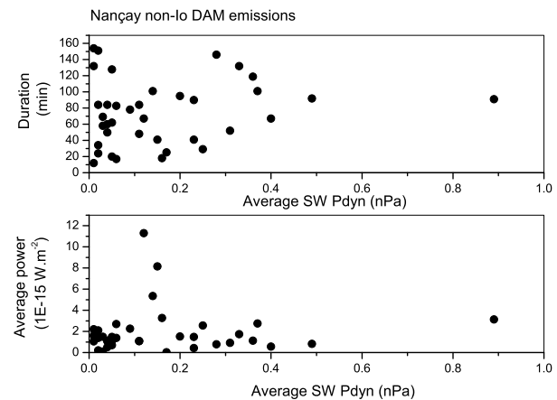
Fig. 7. Scatter plot between Nançay non-Io DAM emission duration and average power versus solar wind dynamic pressure.
