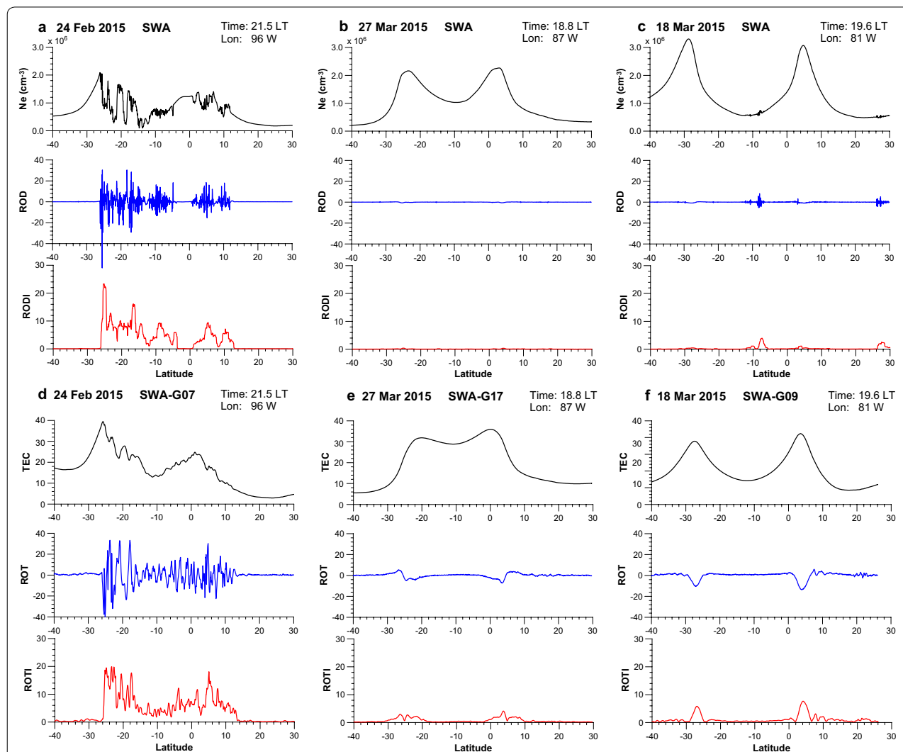
Fig. 3 Examples of the concurrent LP and GPS data analysis during evening LT period for cases of the plasma irregularities detection ( a, d ), quiet-time equatorial ionization anomaly ( b, e ), storm-enhanced equatorial ionization anomaly ( c, f ). Mark like “SWA-G07” means the data along line-of-sight between SWA and GPS PRN 7. TEC data are the relative slant TEC measurements. Detrended ROT/RODI are shown in units of TECU/min, ROD/RODI—in units of 10^6 el/(cm 3 min)
