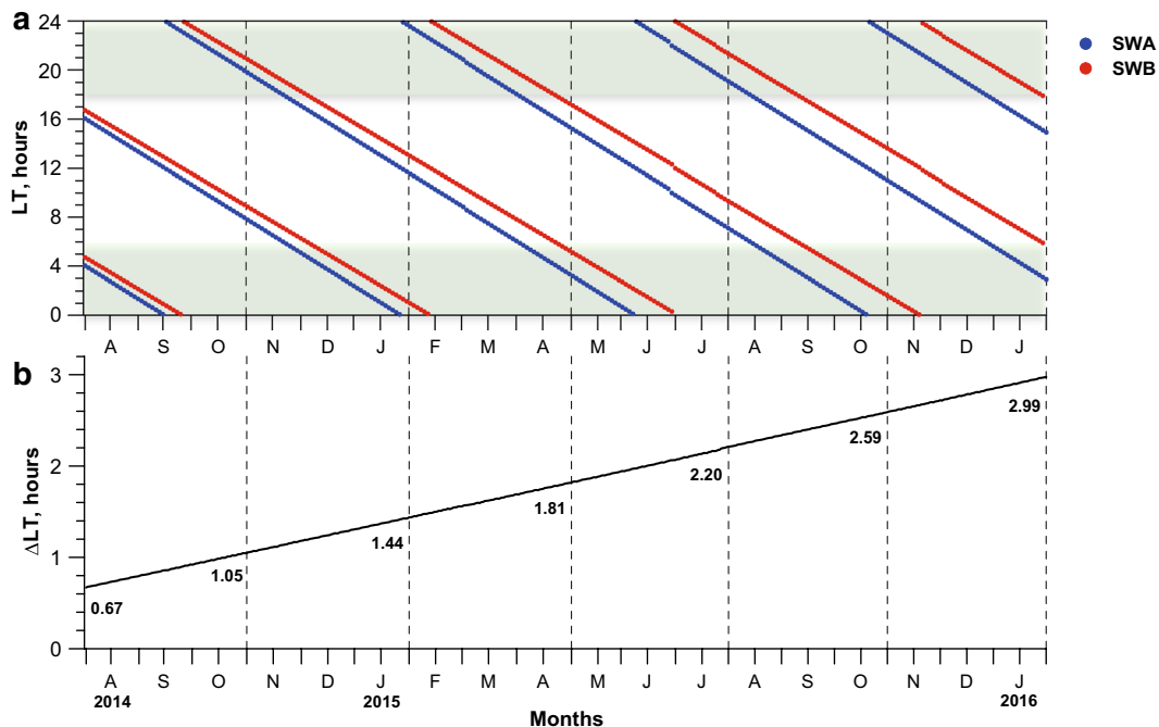
Fig. 1 Temporal difference between SWA/SWB satellites from August 2014 till January 2016: a LT coverage during the considered seasons and LT satellite separation, b progressive time shift in hours between satellites. Minutes are indicated in decimal format. Months are marked by the first letter of their names. Gray shadows indicate a post-sunset interval of 18–06 LT, when equatorial plasma irregularities often occur
