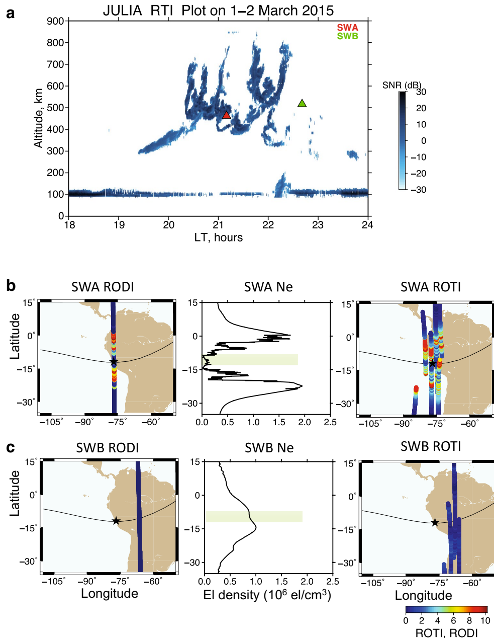
Fig. 6 Example of the post-sunset irregularities occurrence: a spread F echo registered by the JULIA radar in Jicamarca ( 11.7^{\circ}\text{S} ; 78^{\circ}\text{W} ) on March 1–2, 2015, with superimposed position of SWA and SWB overpasses marked by red and green triangles, respectively; latitudinal profiles of RODI, Ne and ROTI for b SWA and c SWB satellites. Light green bars over Ne profiles show latitude of the Jicamarca station. Black asterisk on the ROTI and RODI maps marks the Jicamarca location
