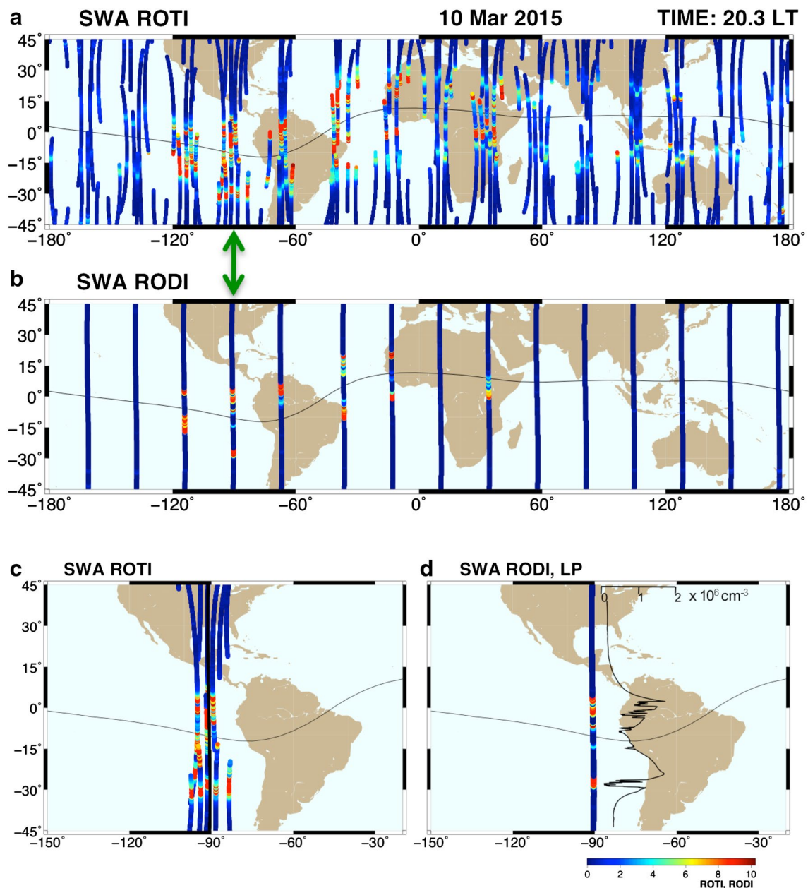
Fig. 2 Comparison of Swarm ROTI and RODI variations for the SWA ascending passes (~20.3 LT) on March 10, 2015. a ROTI values along all separated links Swarm-to-GPS; b RODI values along Swarm track; example of c ROTI and d RODI variation extracted from general maps, which marked by green narrow, and superimposed in situ Ne values as measured by the Swarm LP. Black thin line depicts the geomagnetic equator
