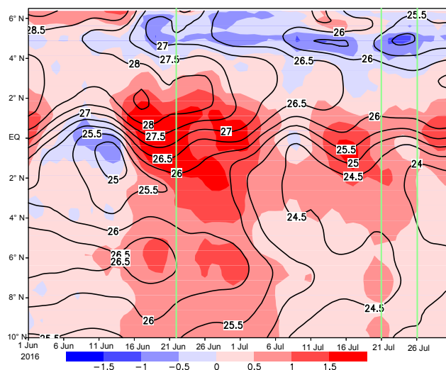
Figure 3. Daily SST behaviour over the eastern tropical Atlantic during June–July 2016. SSTs ( ^{\circ}\text{C} ) are averaged between 10^{\circ}\text{W} and 4^{\circ}\text{E} (see box in Fig. 2) and shown as absolute values (lines) and anomalies (shading). Basis is the Reynolds Optimal Interpolated SST dataset and anomalies are relative to 1981–2016 as in Fig. 2. Only values greater than the SST Reynolds daily error estimation are plotted. The four phases of the DACCIWA campaign are marked with thin green lines.
