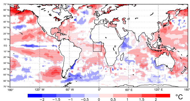
Figure 2. Global SST anomalies for June–July 2016 ( ^{\circ}\text{C} ). Basis is the Reynolds Optimal Interpolated SST v2 dataset and anomalies are relative to 1981–2016. Only anomalies above the 95 % confidence level based on a two-sided Student's t test are plotted. The black box marks the area used for Fig. 3.
